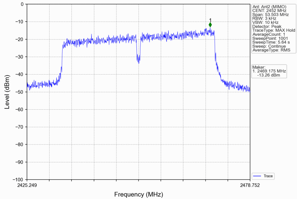
802.11ax(HEW40)_HCH_2452MHz_RU484_Left_MIMO_NTNV
