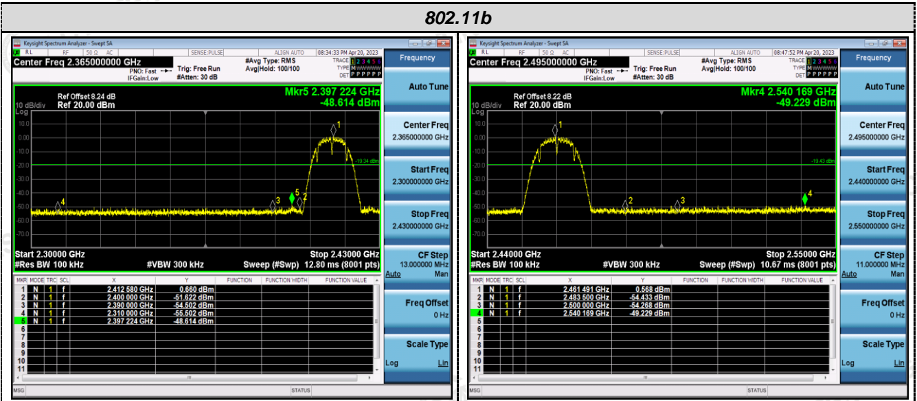
Left bandedge
