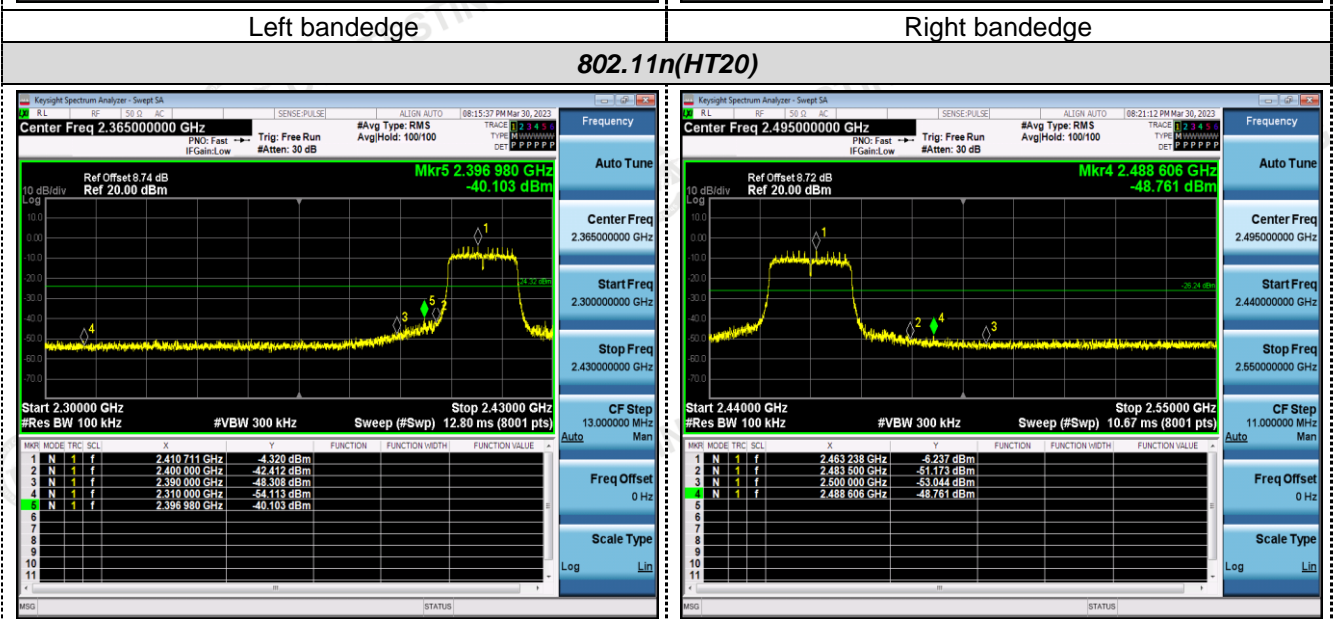
Left bandedge
