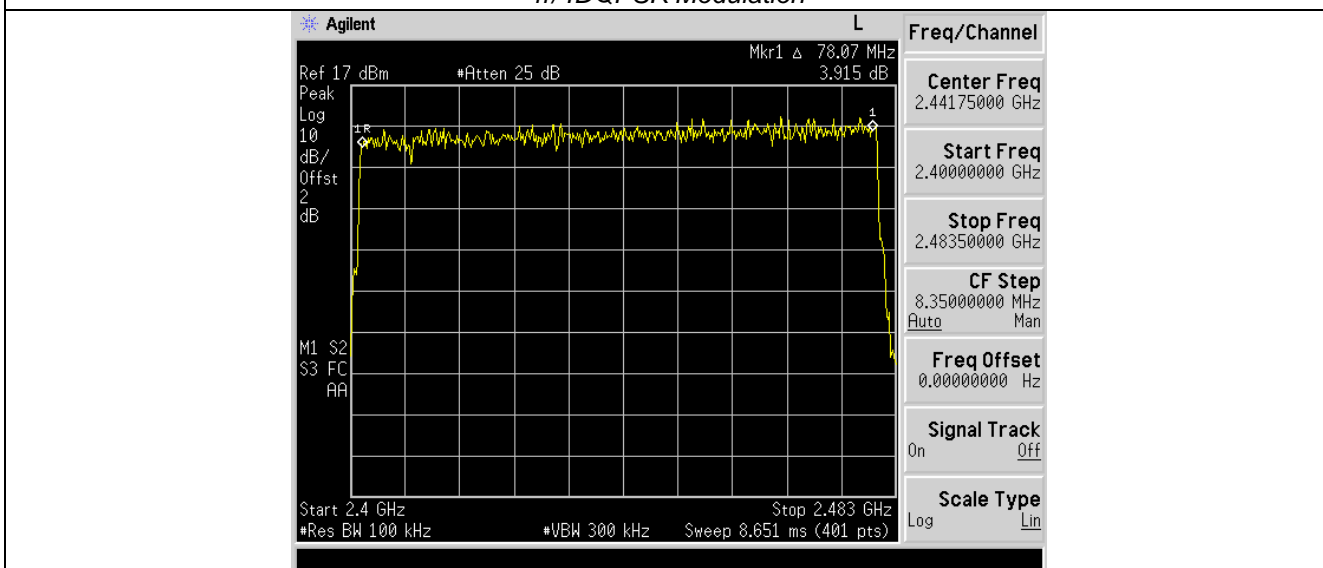
8DPSK Modulation
