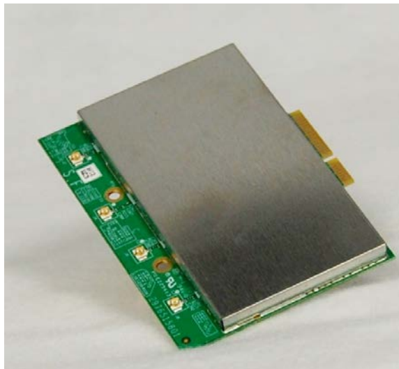
Figure 1 - Top View of the 802.11ac WiFi Radio Module - U.FL connectors
