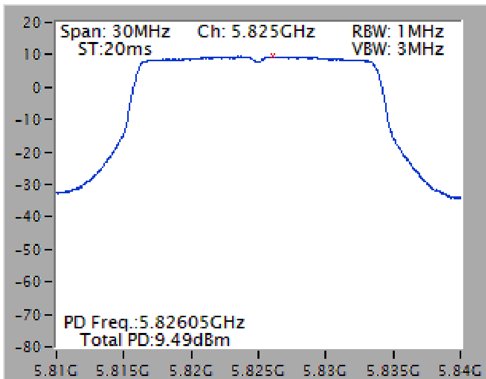
Power Density Plot on Configuration IEEE 802.11ac MCS0/Nss1 VHT20 / Chain 1 + Chain 2 + Chain 3 + Chain 4 / 5825 MHz
