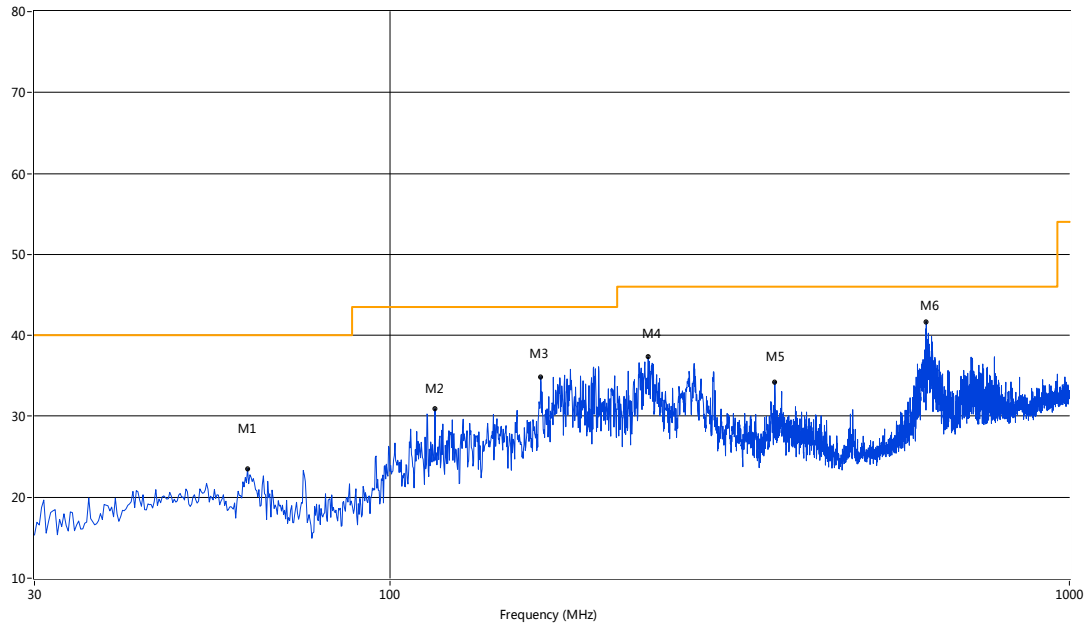
RE Test case_FCC_Part 15C_FCC 15C 30MHz-1GHz
