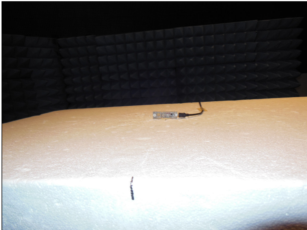
Figure 2: Radiated Emissions - Attached Eval Board
