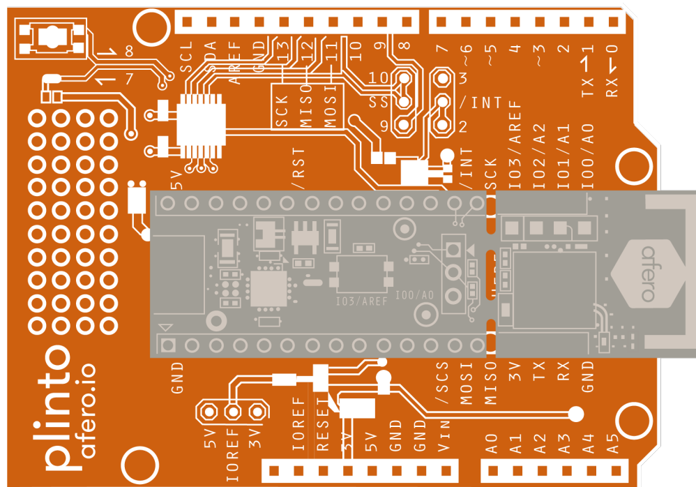
Modulo-Plinto connections
