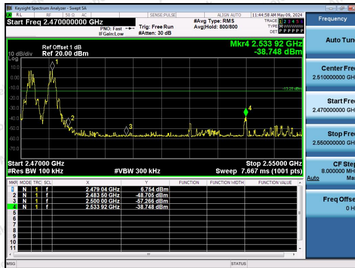
2.4G-Ant1-Hop_2479-PASS
