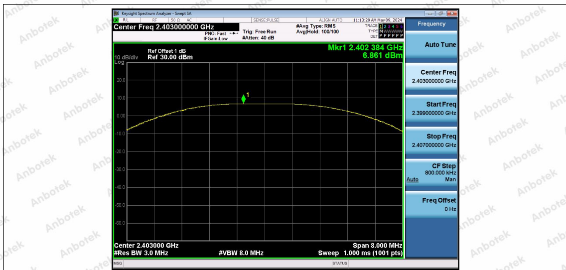
2.4G-Ant1-2403-PASS
