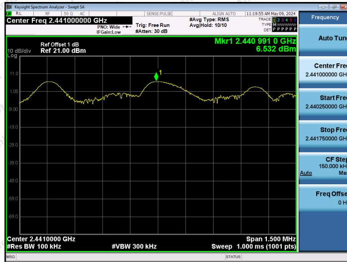
2.4G-Ant1-2441-0~Reference-PASS
