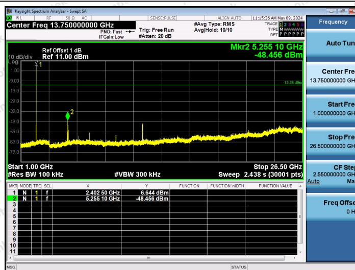
2.4G-Ant1-2403-1000~26500-PASS
