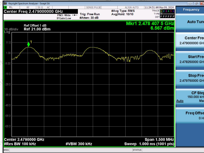
2.4G-Ant1-2479-0~Reference-PASS
