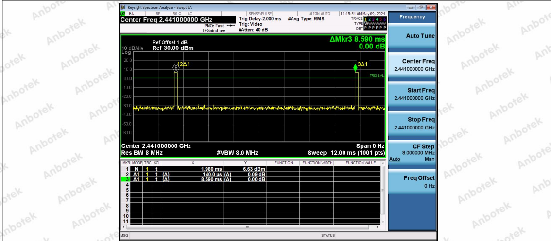
NTNV-2.4G-Ant1-2441
