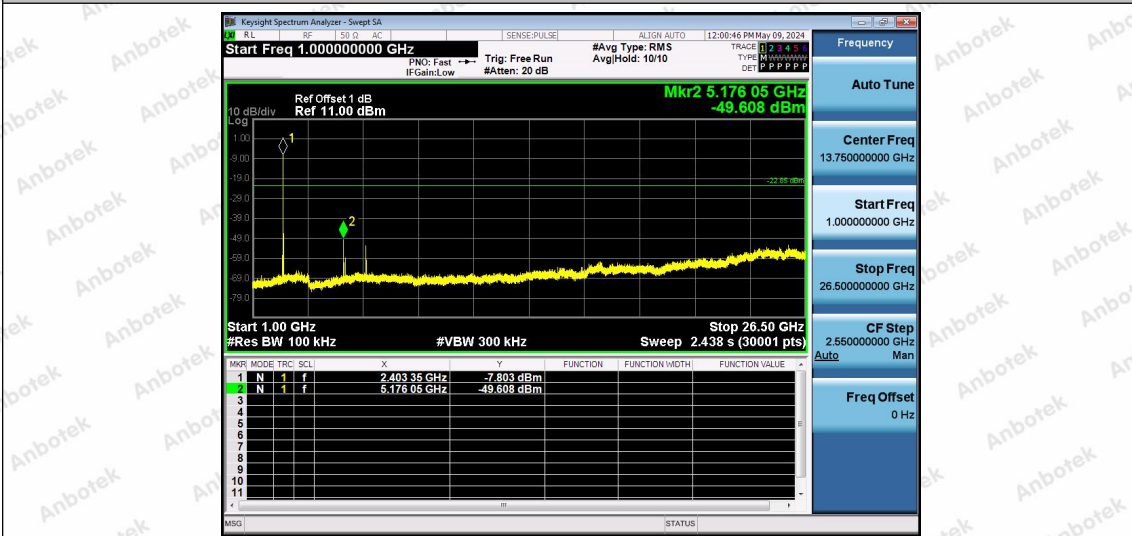
2.4G-Ant1-2403-1000~26500-PASS
