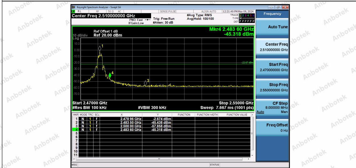
2.4G-Ant1-2479-PASS
