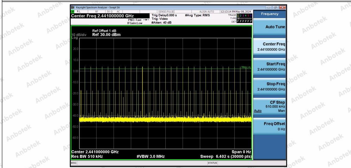
2.4G-Ant1-Hop-PASS
