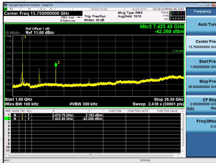
2.4G-Ant1-2474-1000~26500-PASS
