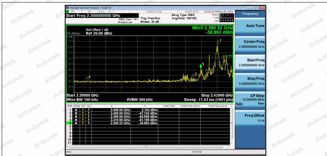
2.4G-Ant1-2408-PASS
