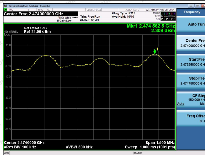
2.4G-Ant1-2474-0~Reference-PASS
