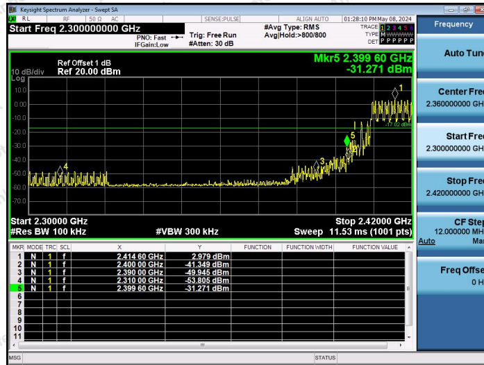
2.4G-Ant1-Hop_2408-PASS
