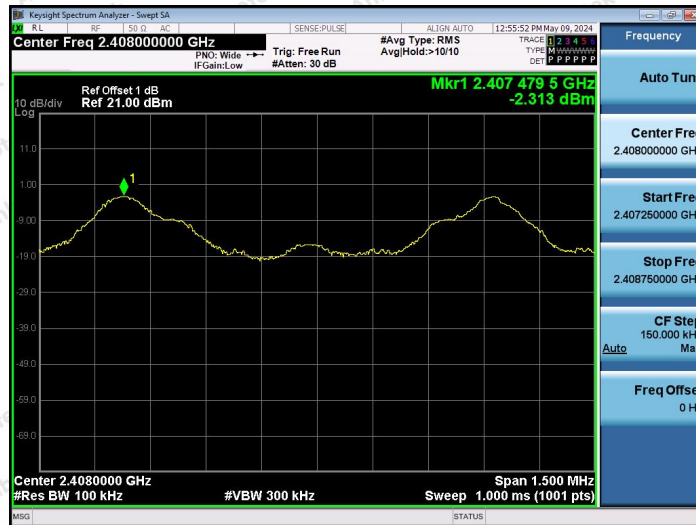
2.4G-Ant1-2408-0~Reference-PASS
