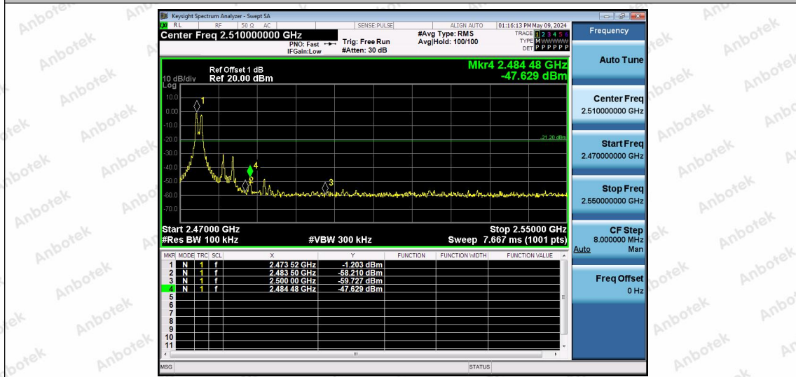
2.4G-Ant1-2474-PASS
