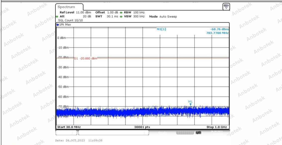
2.4G_Ant1_2437_30~1000
