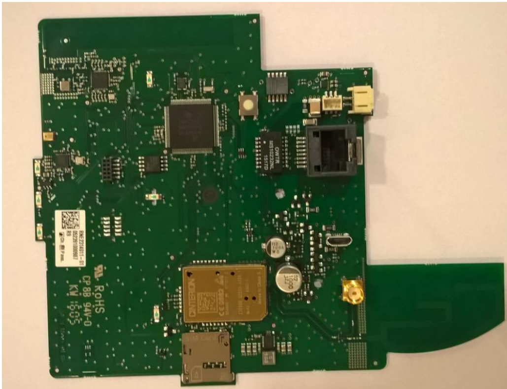
NOVO IP PCB, TOP
