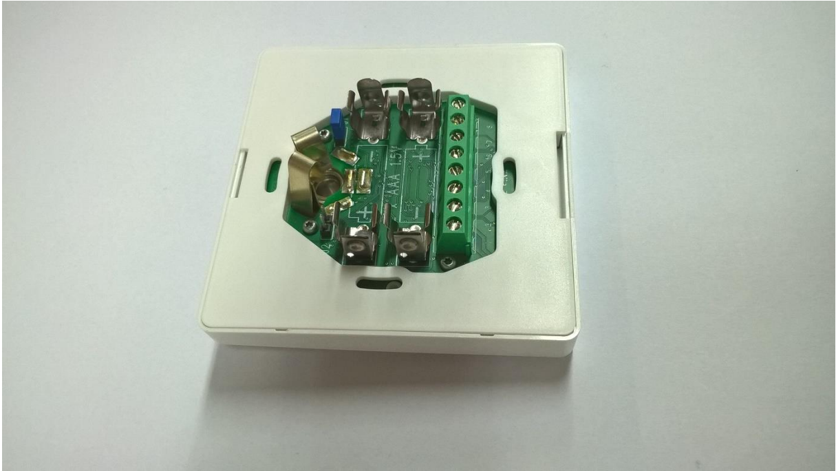
3PUSH+PEAR BACK SIDE VIEW
