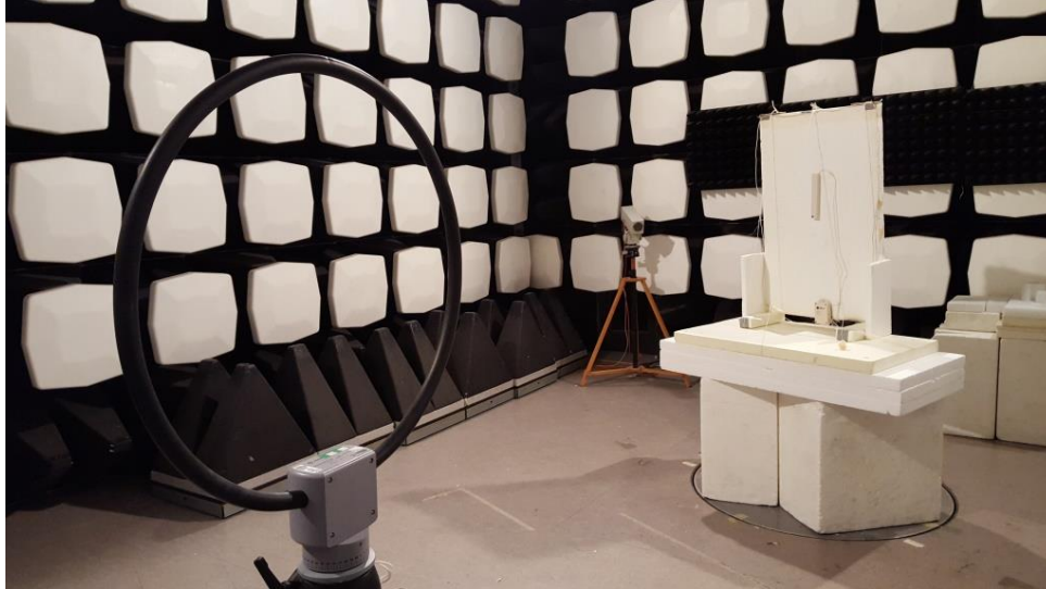
9 kHz-30 MHz, semi anechoic chamber, loop antenna, antenna pos C
