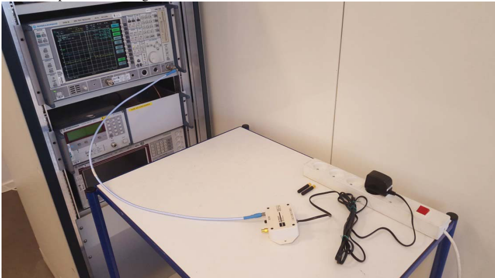
Test set up for Band Edge, 20 dB BW and OBW measurements
