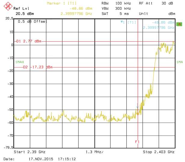
Hopping mode
