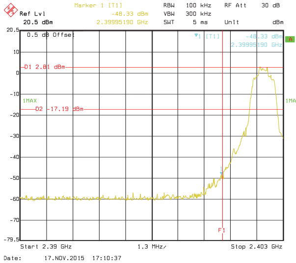
No-hopping mode
