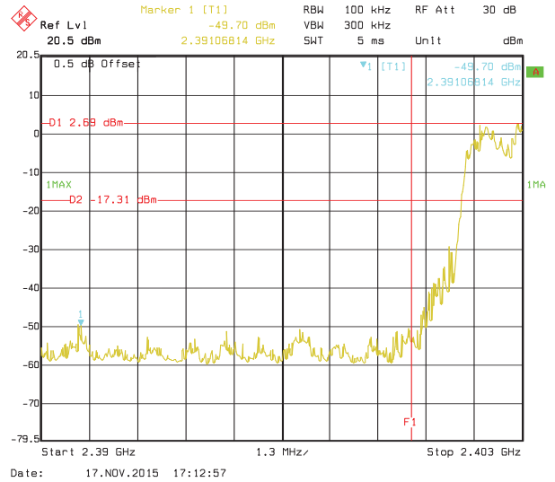
Hopping mode
