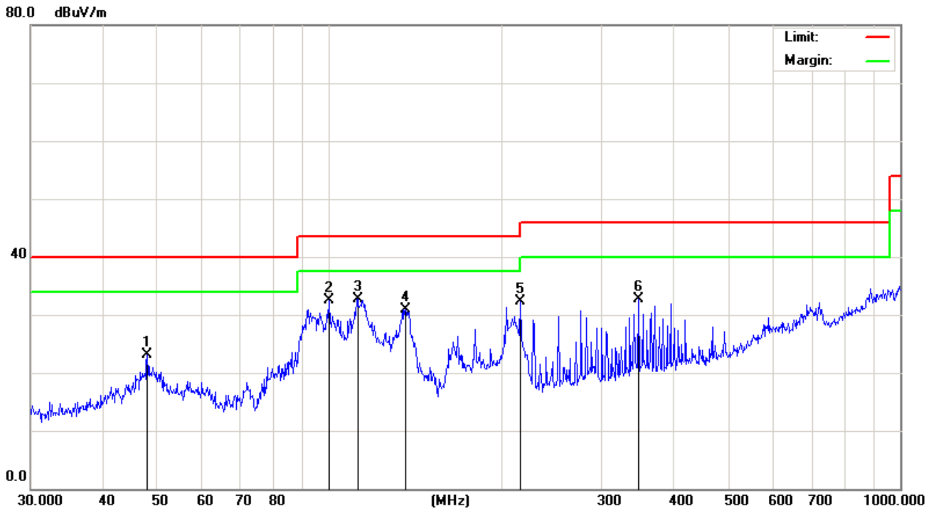
Quasi-peak measurement
