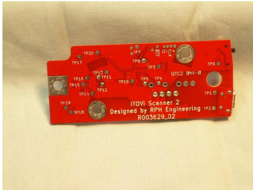
Photograph 13 – View of the Trace Side of the PCB
