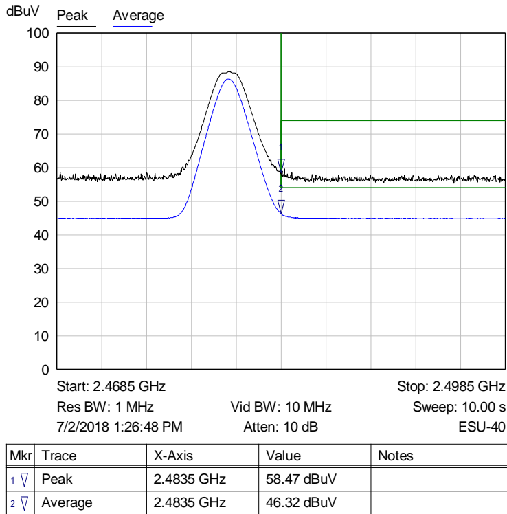
Graph 8: Radiated Upper Band Edge Plot
