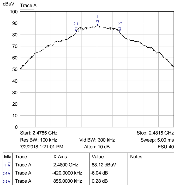
Graph 3: Highest Channel Bandwidth
