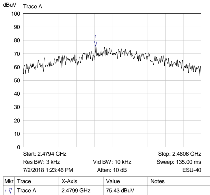
Graph 11: Highest Channel Output 3 kHz PSD Plot
