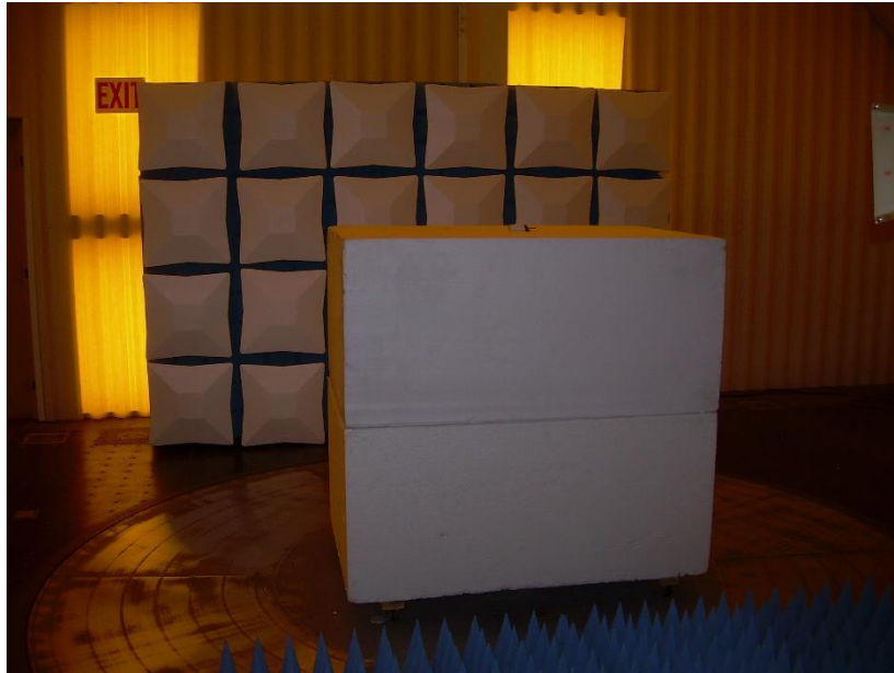
Photograph 3 – Front View Radiated Emissions – Above 1000 MHz
