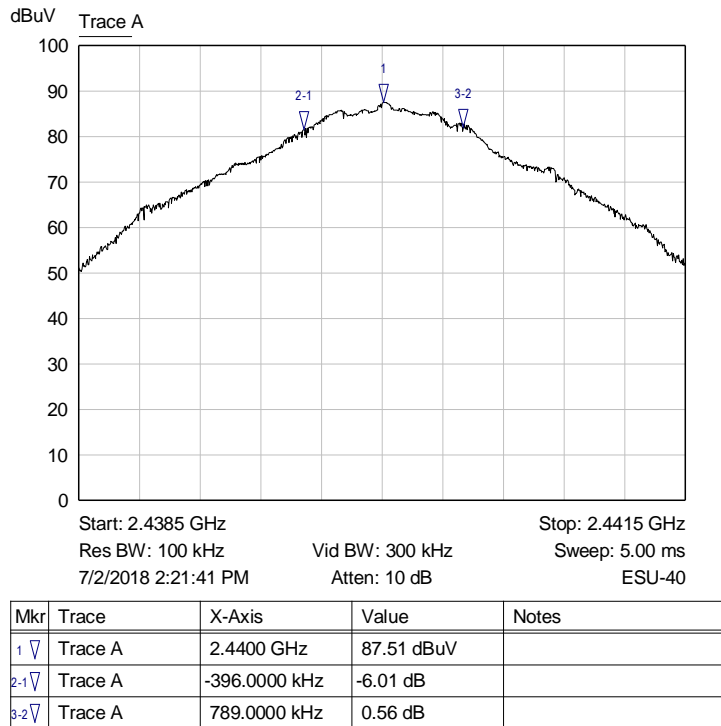
Graph 2: Middle Channel Bandwidth
