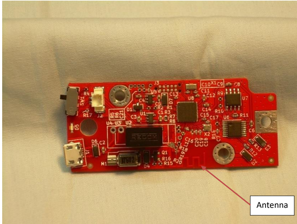
Photograph 1 – Top View of the Component Side of the PCB
