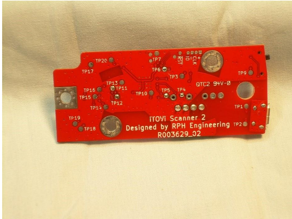
Photograph 2 – View of the Trace Side of the PCB
