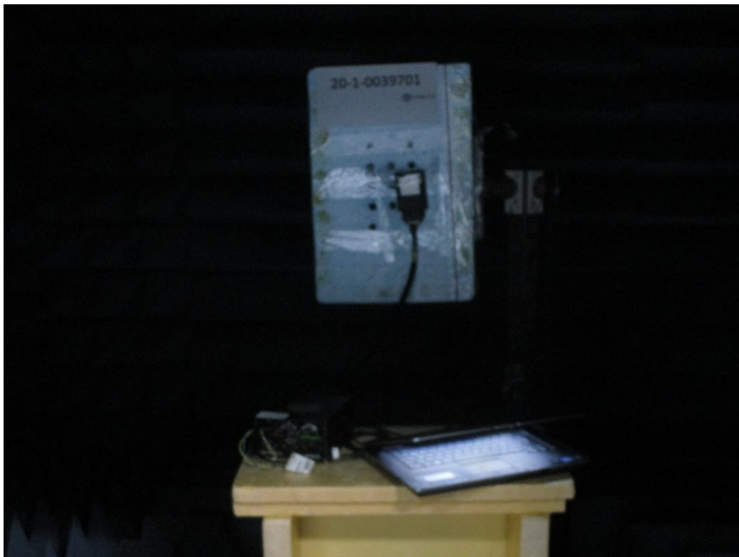
Fig. Mea.: 4 : Radiated Emission setup above 1GHz
