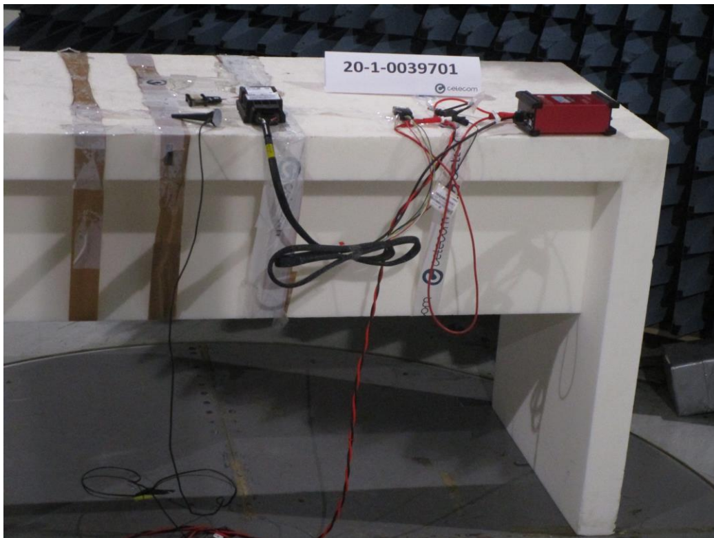
Fig. Mea.: 2 : Radiated Emission setup below 1GHz
