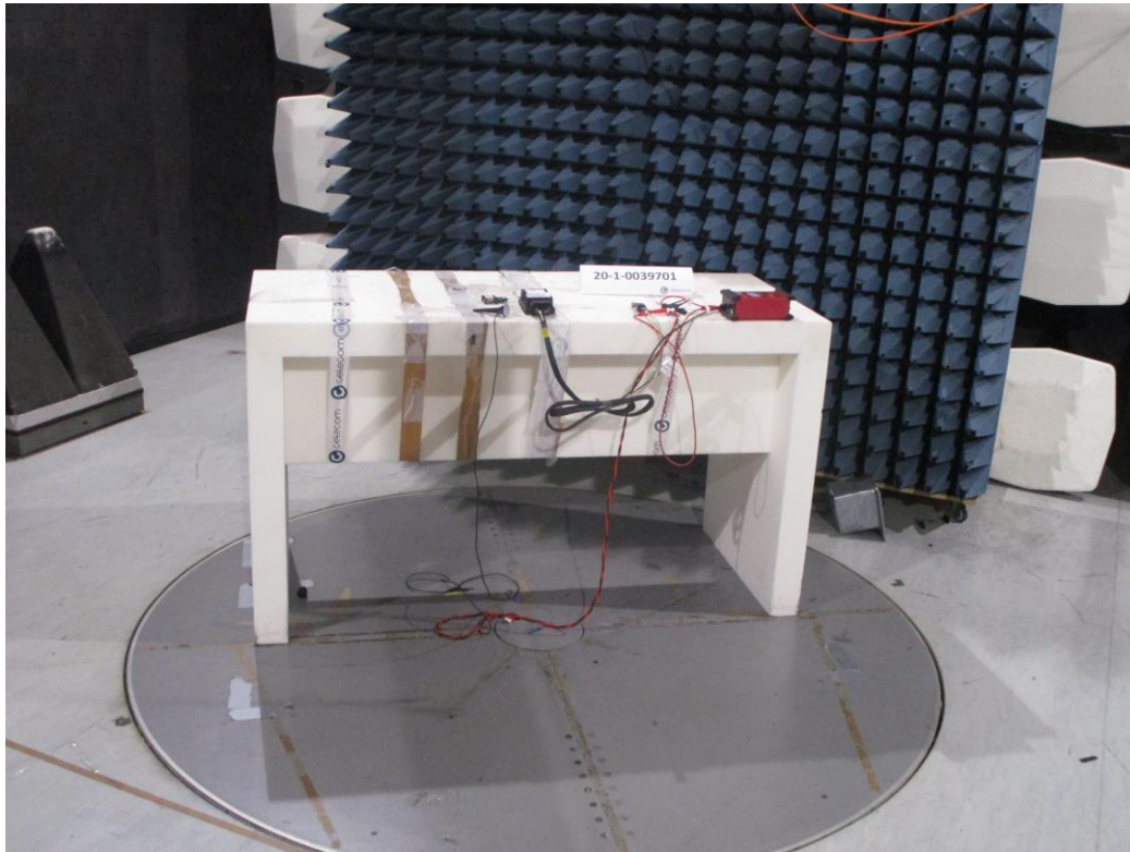
Fig. Mea.: 1 : Radiated Emission setup below 1GHz
