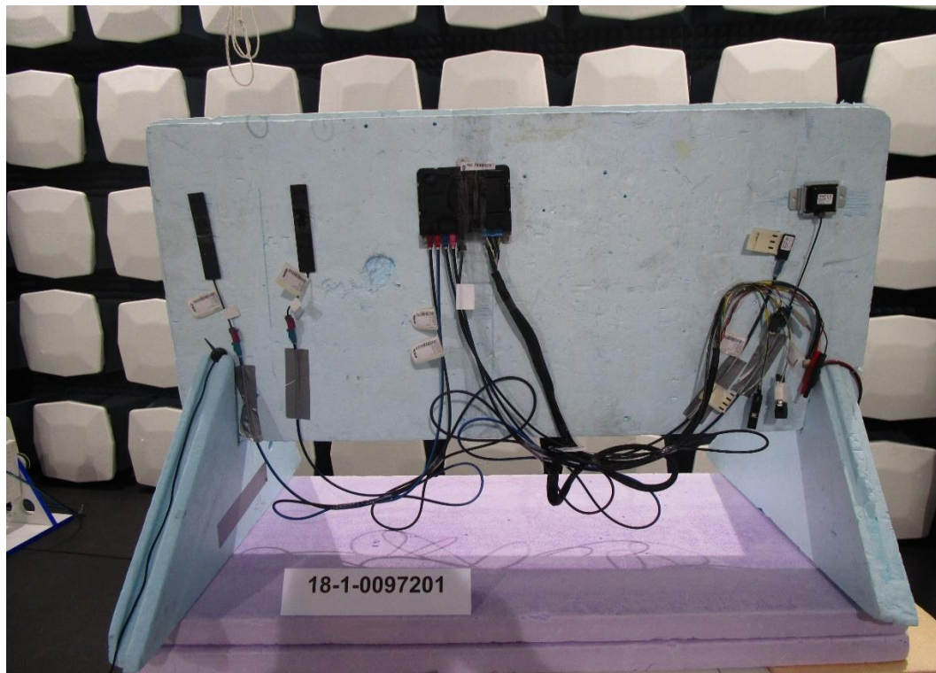
Photograph 2: EUT standing: close view
