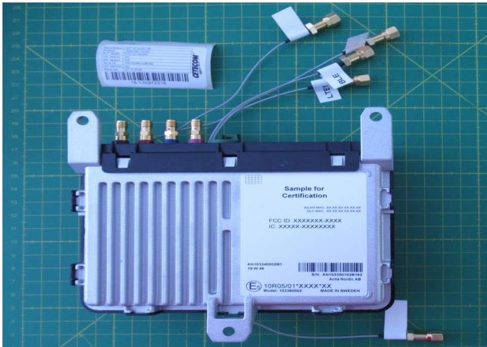
Photograph 7: EUT B_Rear side view
