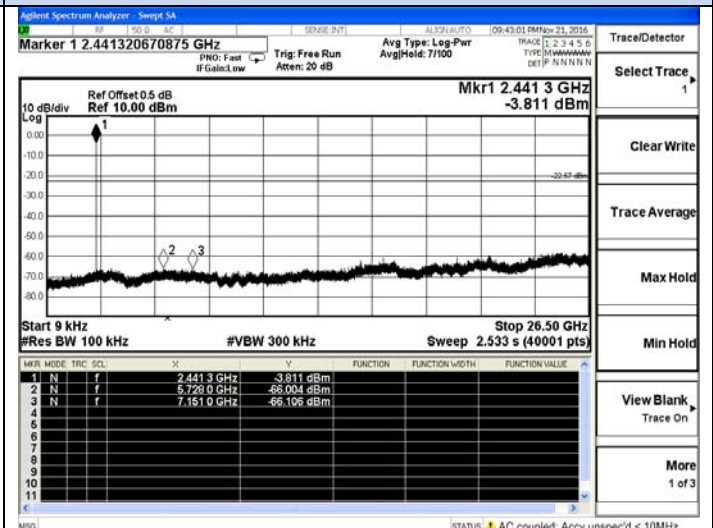
3DH1-Middle channel
