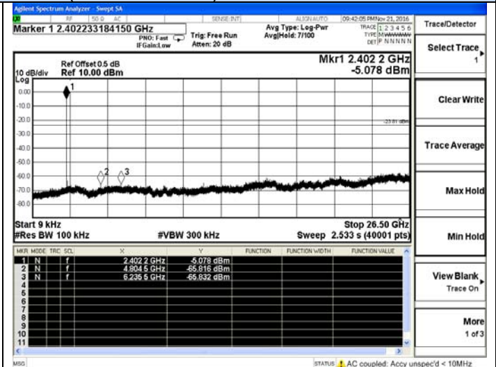
3DH1-Low channel
