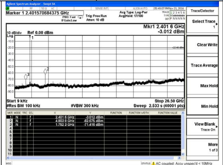
DH1-Low channel
