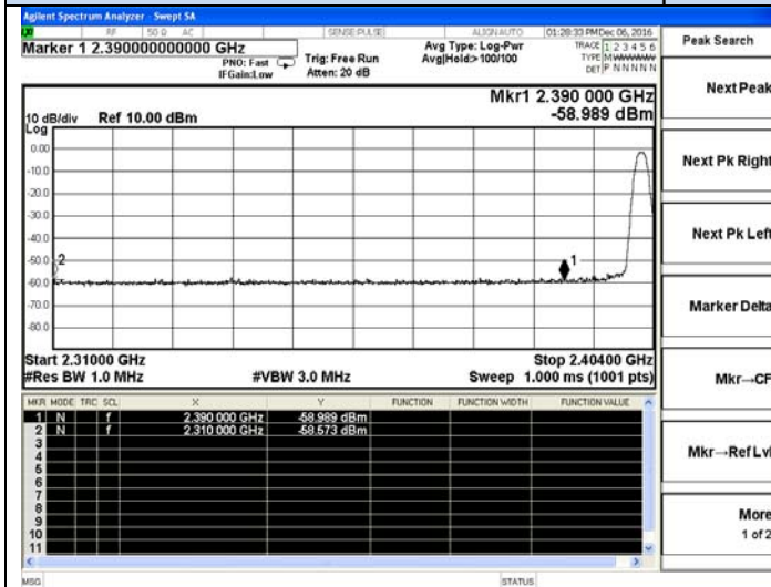
GFSK-Low channel(Peak)
