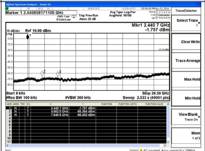
DH1-Middle channel
