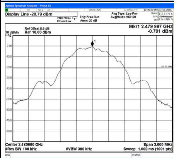
BT LE-High channel Reference
