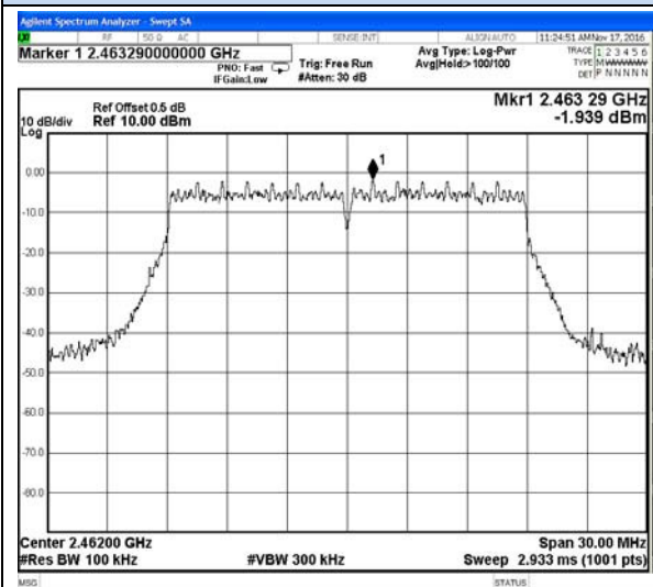
IEEE 802.11n(HT20)-High channel Reference
