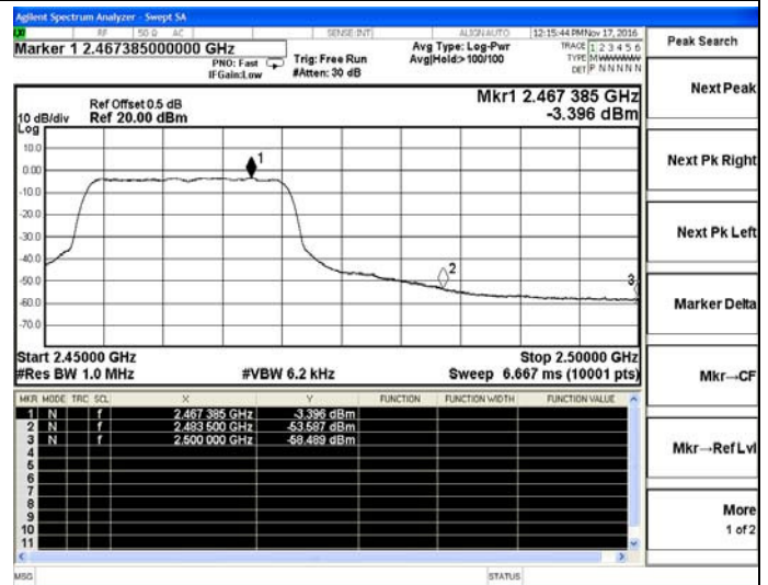
802.11g-High channel(Average)
