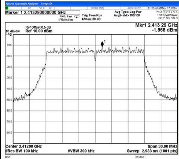
IEEE 802.11n(HT20)-Low channel Reference
