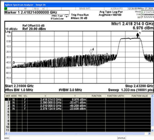
802.11n(HT20)-Low channel(Peak)
