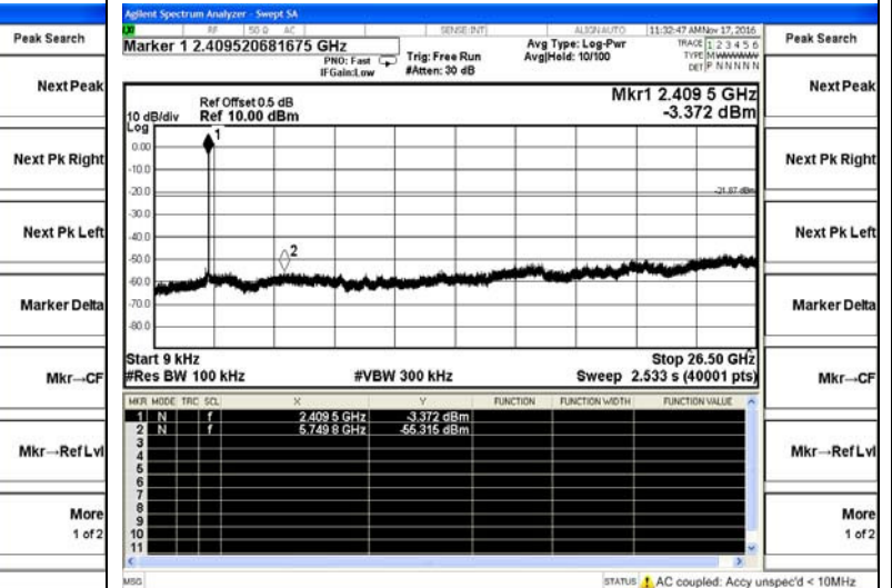
IEEE 802.11n(HT20)-Low channel
