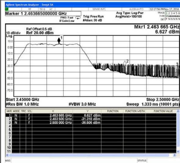
802.11g-High channel(Peak)
