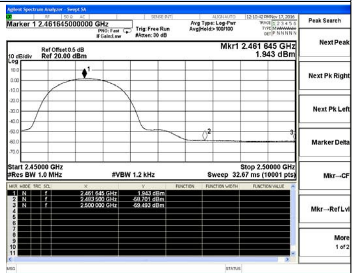
802.11b-High channel(Average)
