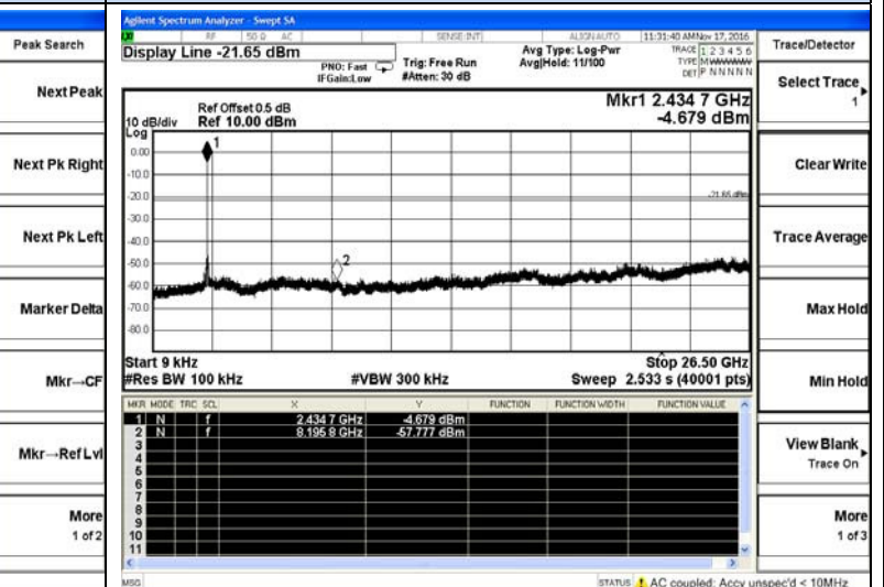
IEEE 802.11n(HT20)-Middle channel
