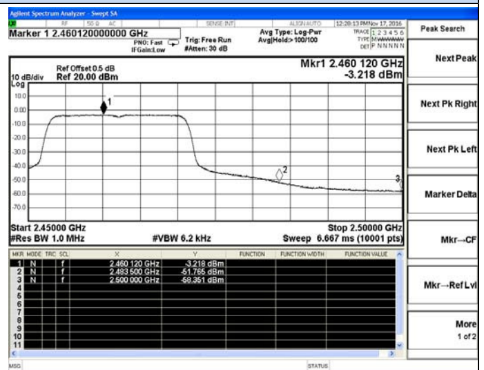
802.11n(HT20)-High channel(Average)
