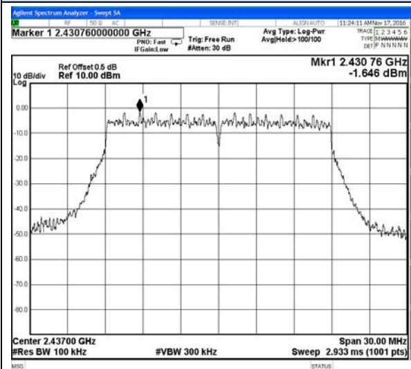
IEEE 802.11n(HT20)-Middle channel Reference
