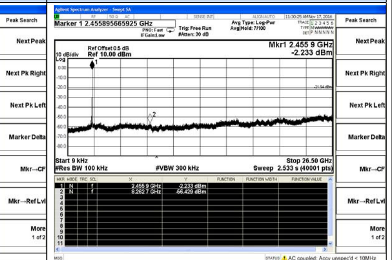
IEEE 802.11n(HT20)-High channel
