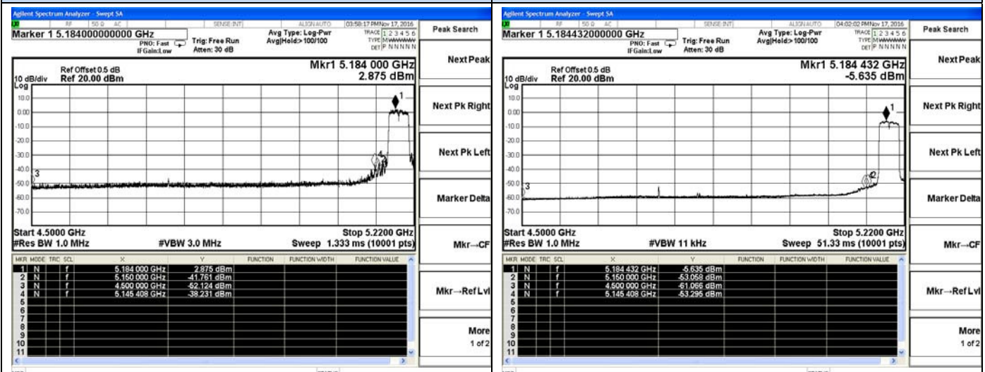
802.11n-HT40-Low channel(Peak)
