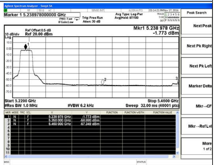
802.11a-High channel(Average)
