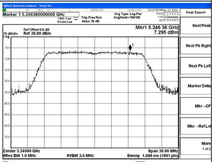
IEEE 802.11n-HT20-5240MHz
