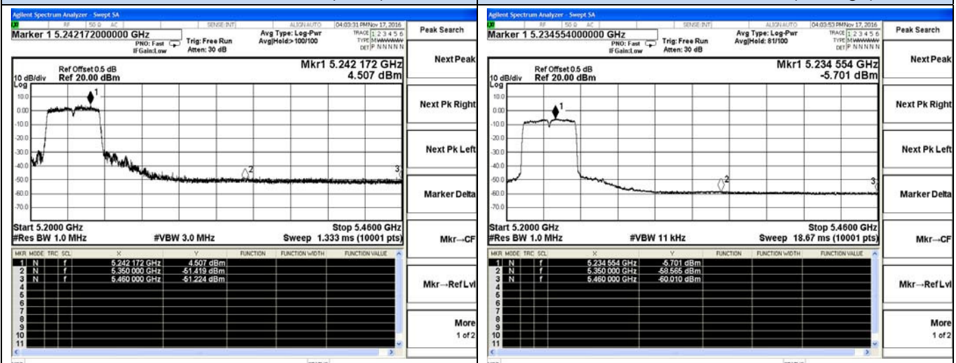
802.11n-HT40-High channel(Peak)
