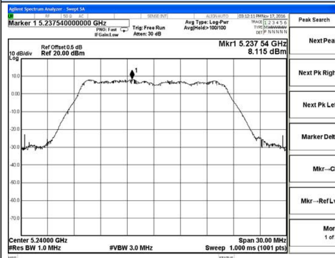
IEEE 802.11a-5240MHz
