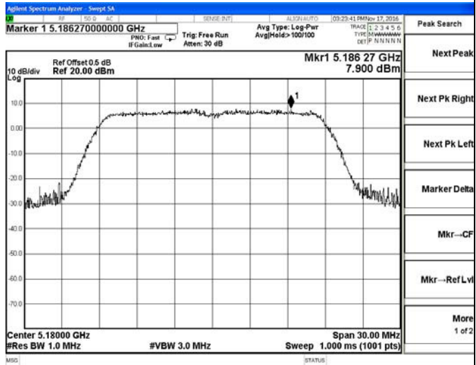
IEEE 802.11n-HT20-5180MHz
