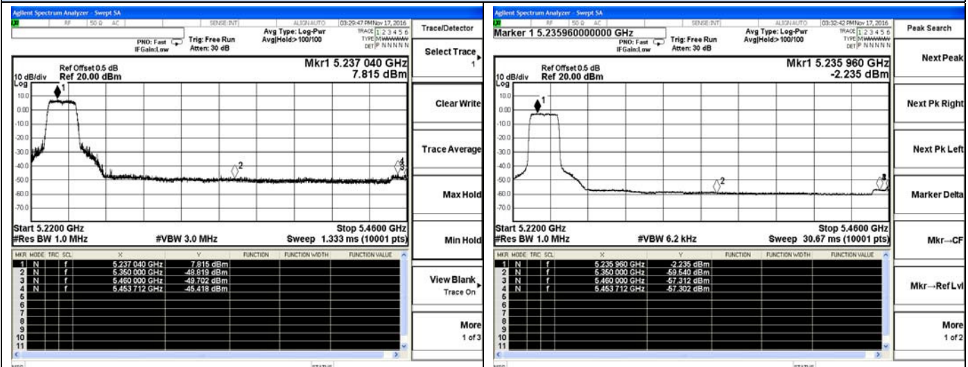
802.11n-HT20-High channel(Peak)
