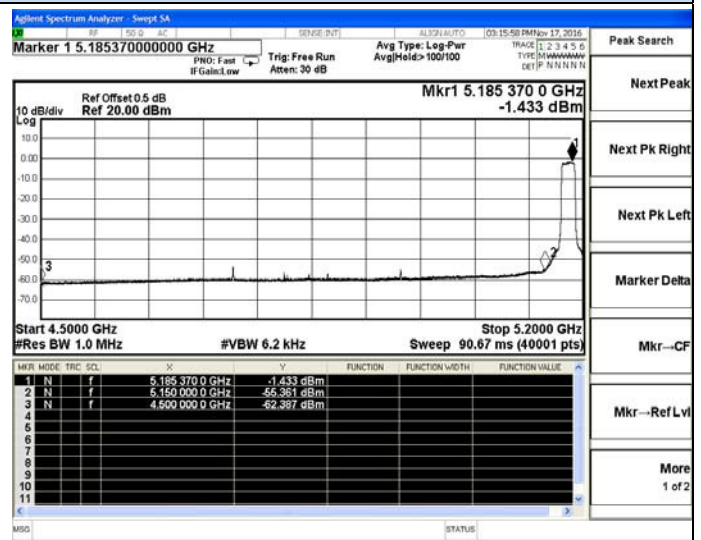
802.11a-Low channel(Average)
