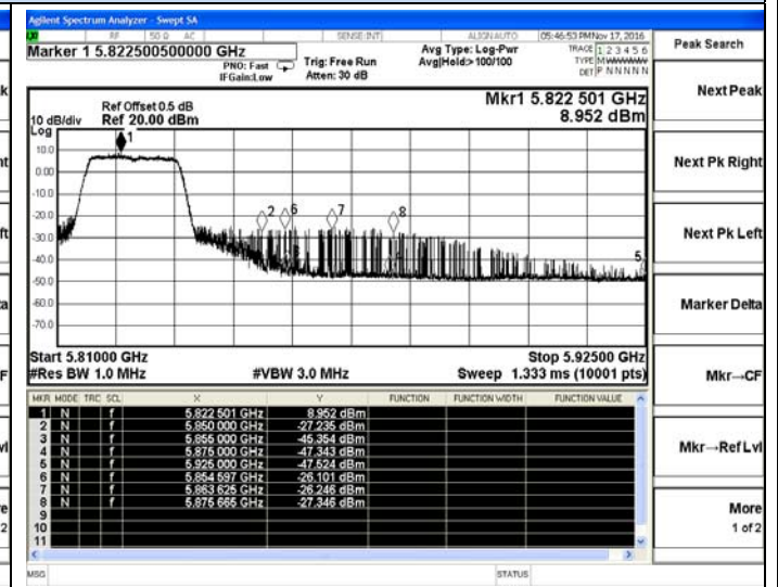
IEEE 802.11ac VHT20-High channel(Peak)
