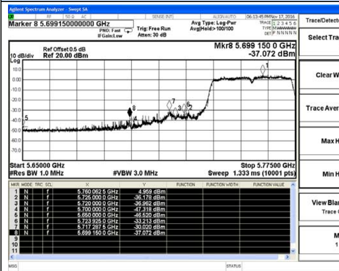
IEEE 802.11ac VHT40-Low channel(Peak)
