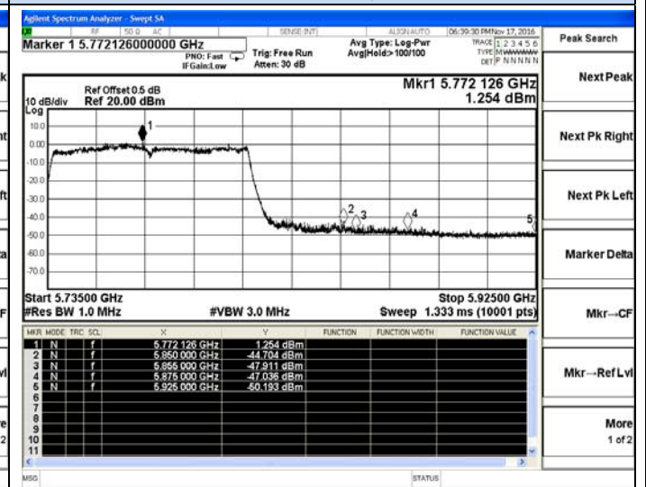
IEEE 802.11ac VHT80-High channel(Peak)
