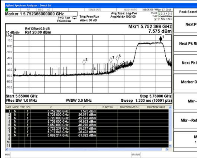
IEEE 802.11ac VHT20-Low channel(Peak)
