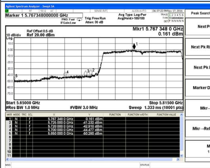
IEEE 802.11ac VHT80-Low channel(Peak)
