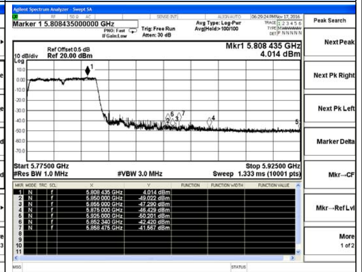
IEEE 802.11ac VHT40-High channel(Peak)
