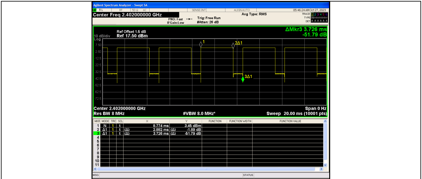
GFSK(DH5)_Channel 0
