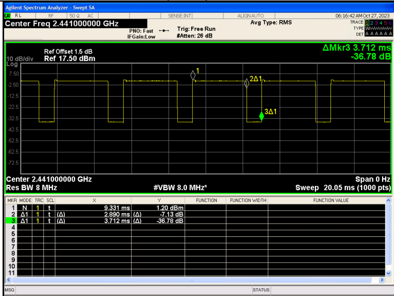
8DPSK(3-DH5) Channel 39
