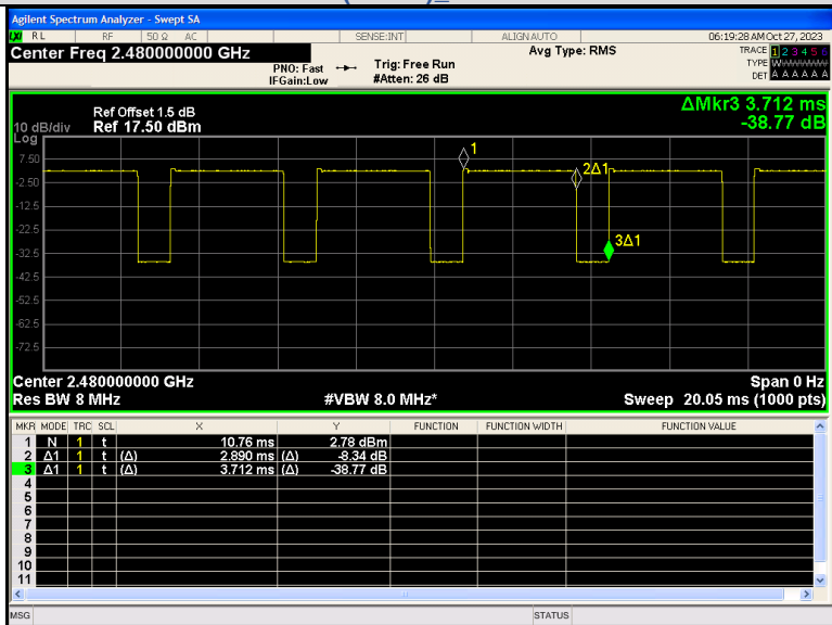
8DPSK(3-DH5) Channel 78
