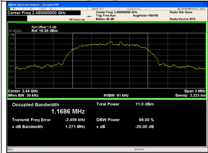
8DPSK_3-DH5_Channel 78
