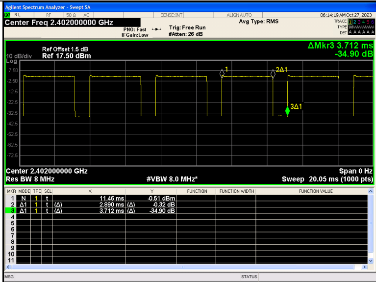
8DPSK(3-DH5) Channel 0
