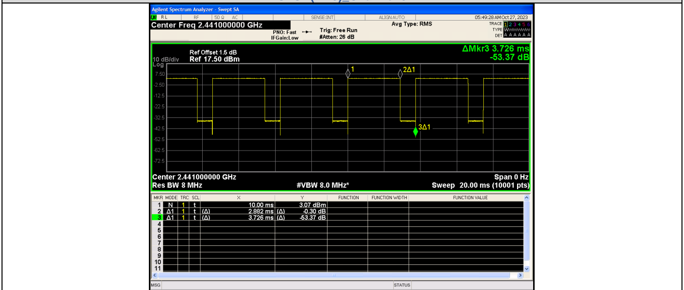
GFSK(DH5)_Channel 39
