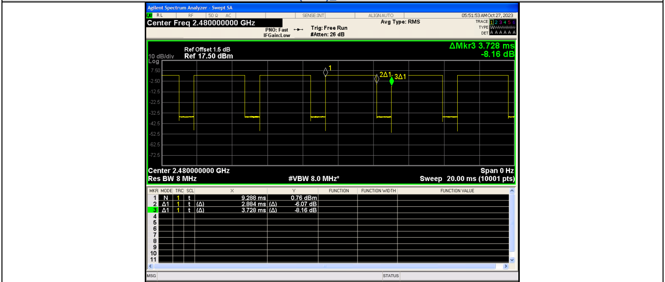
GFSK(DH5)_Channel 78
