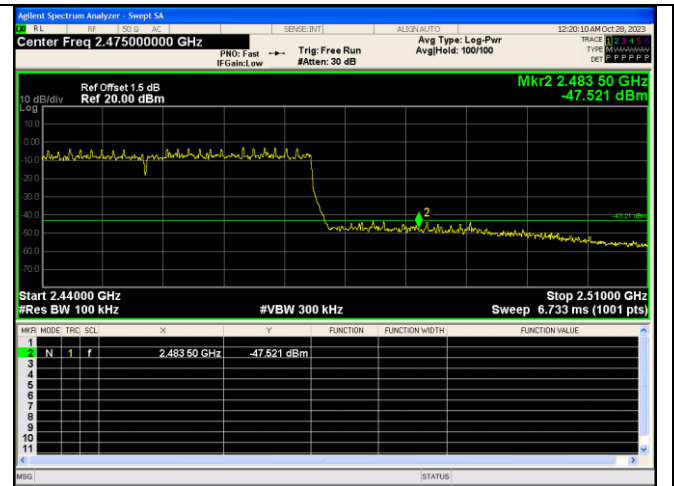
Out Of Band Emission IEEE 802.11ax_Channel 9_40MHz_Antenna 0_RU&Index 484RU65
