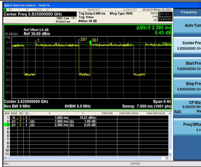
802.11ac(VHT20)_Ant2_5825
