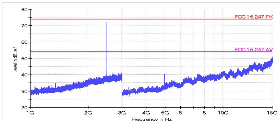
Electric Field Strength FCC 15.247 1-18GHz
