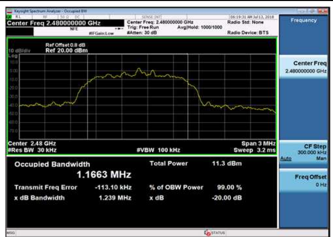
DQPSK,2480MHz,2DH5
