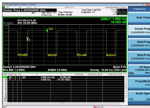
GFSK,2402,DH5,Transmission Time
