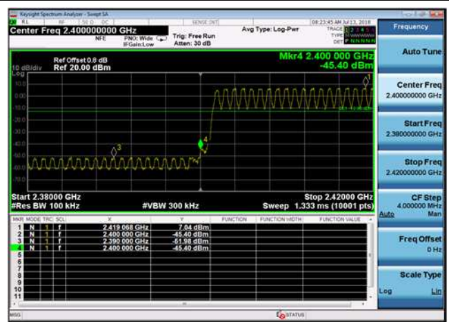
DQPSK,Hopping,2DH5,Band Edge LowRange
