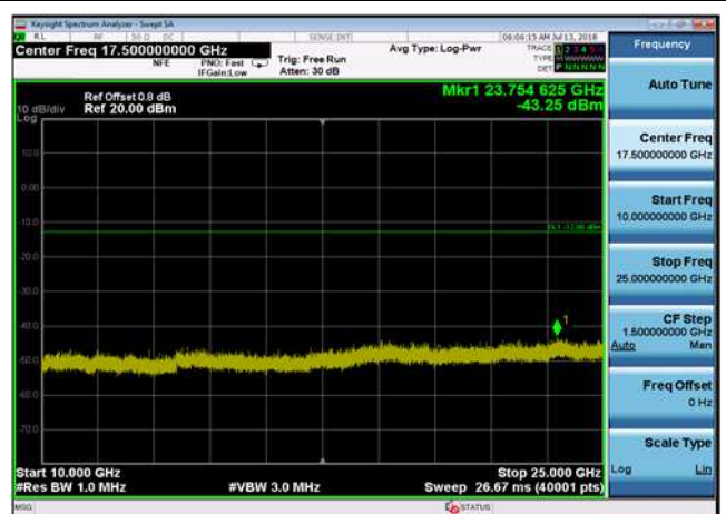
GFSK,2480MHz,DH5,Plot 4,10000MHz~25000MHz
