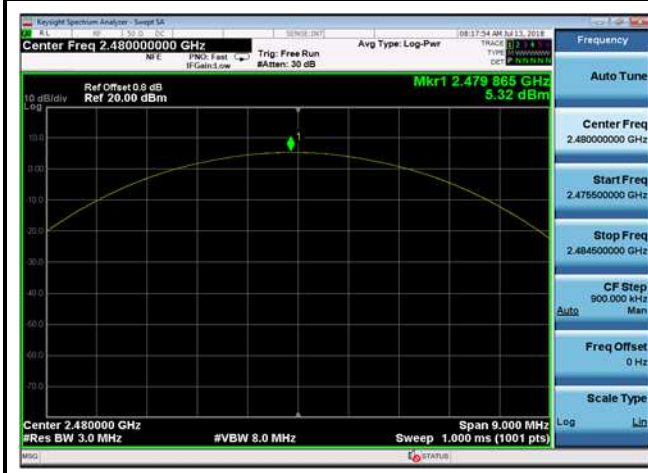
8DPSK,2480MHz,3DH5
