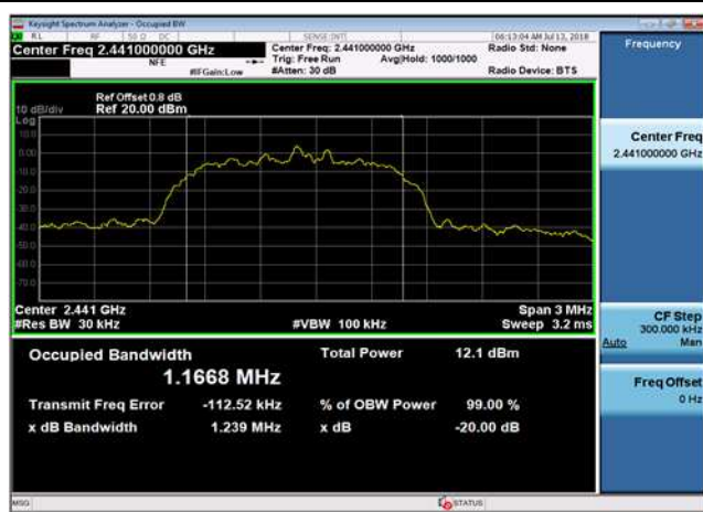
DQPSK,2441MHz,2DH5
