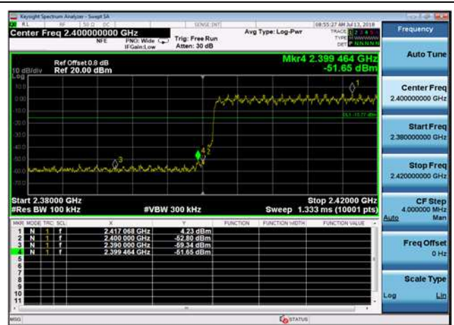
8DPSK,Hopping,3DH5,Band Edge LowRange
