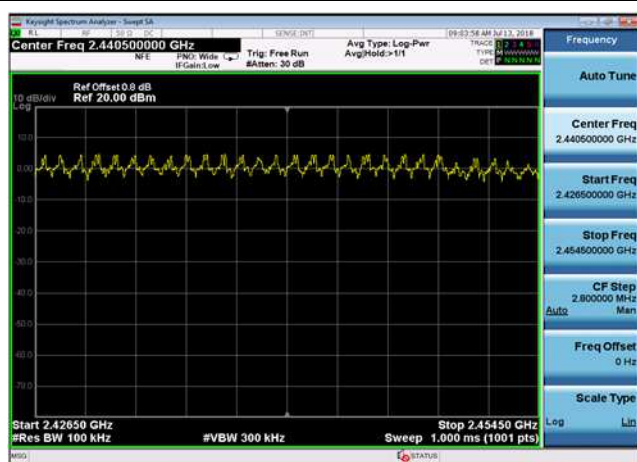
8DPSK,Hopping,3DH5,2426.5~2454.5MHz
