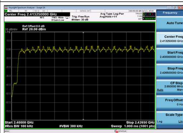
DQPSK,Hopping,2DH5,2400~2426.5MHz
