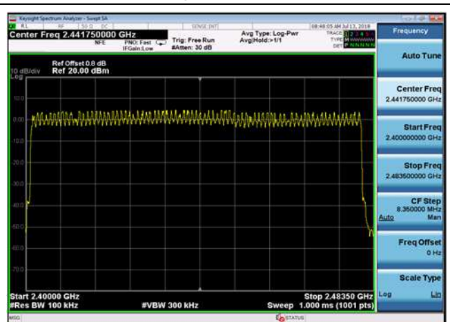
DQPSK,Hopping,2DH5,2400~2483.5MHz
