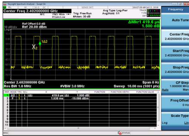
GFSK,2402,DH3,Transmission Time
