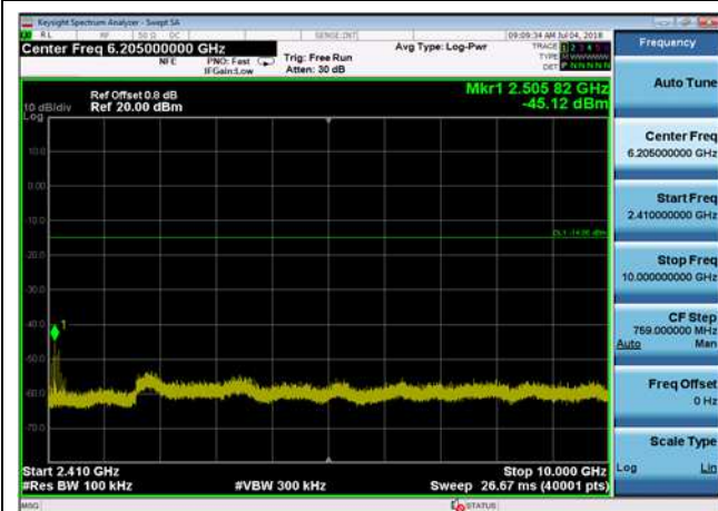
GFSK,2441MHz,DH5,Plot 1,Band Edge
