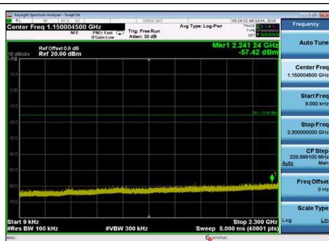
DQPSK,2441MHz,2DH5,Plot 2,0.009MHz~2300MHz
