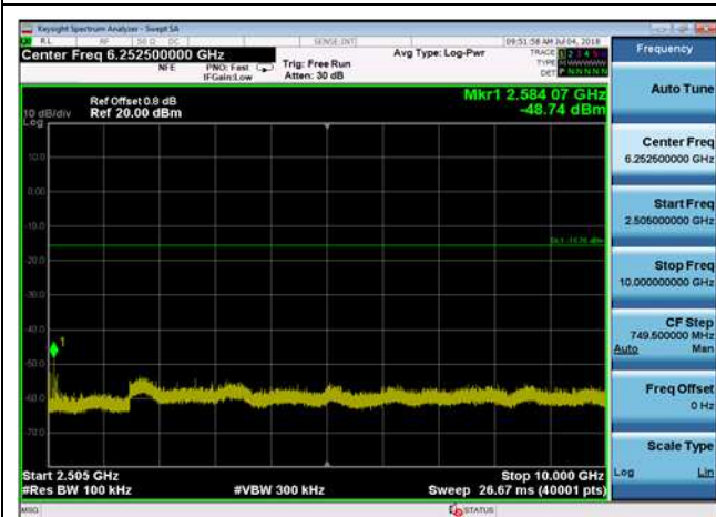
8DPSK,2480MHz,3DH5,Plot 3,2505MHz~10000MHz
