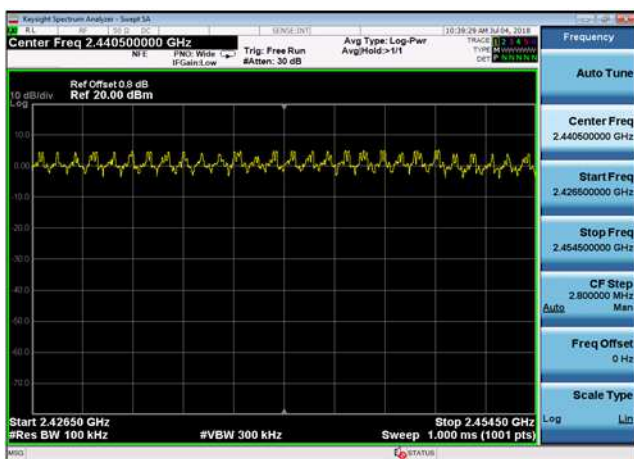
8DPSK,Hopping,3DH5,2426.5~2454.5MHz
