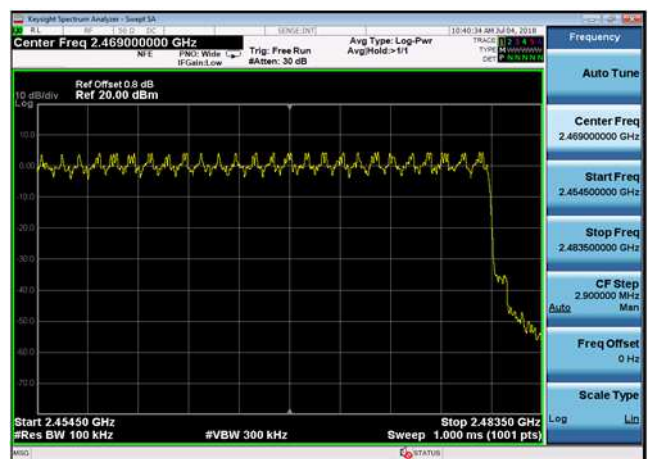
8DPSK,Hopping,3DH5,2454.5~2483.5MHz
