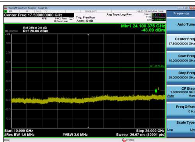
8DPSK,2480MHz,3DH5,Plot 4,10000MHz~25000MHz
