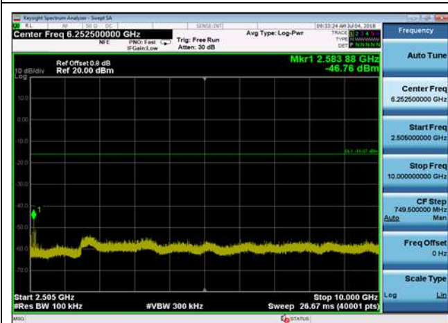
DQPSK,2480MHz,2DH5,Plot 3,2505MHz~10000MHz
