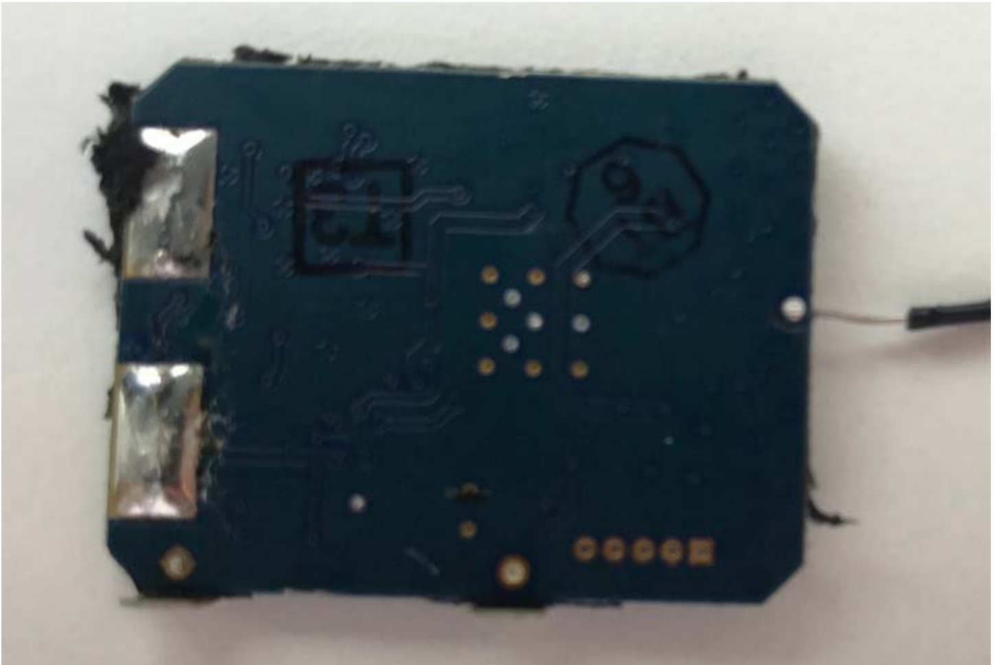
Bottom Detail View of Board with Battery Pack Removed.
