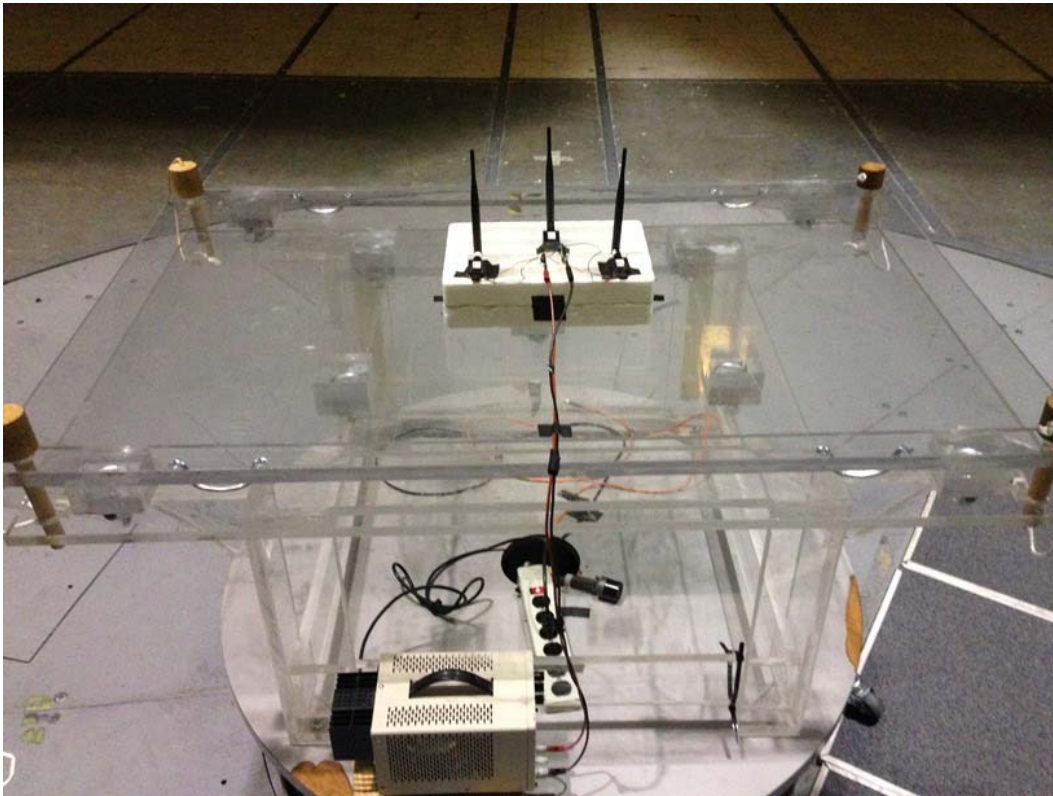
Radiated Spurious, Front
