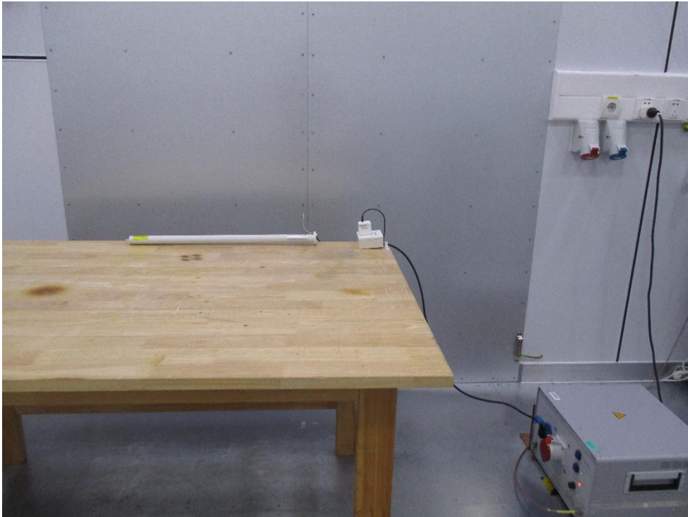
Conduction Emission
