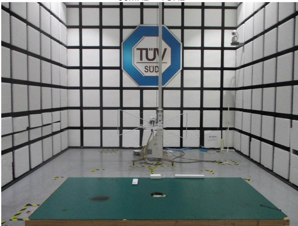
Radiated Emission Setup 30MHz ~ 1GHz
