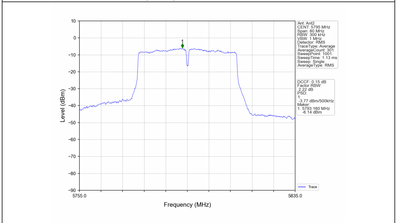
802.11ac(VHT40)_HCH_5795MHz_Ant2_NTNV
