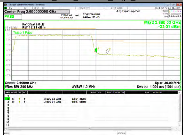
Band41_15M_16QAM_High_Full-RB
