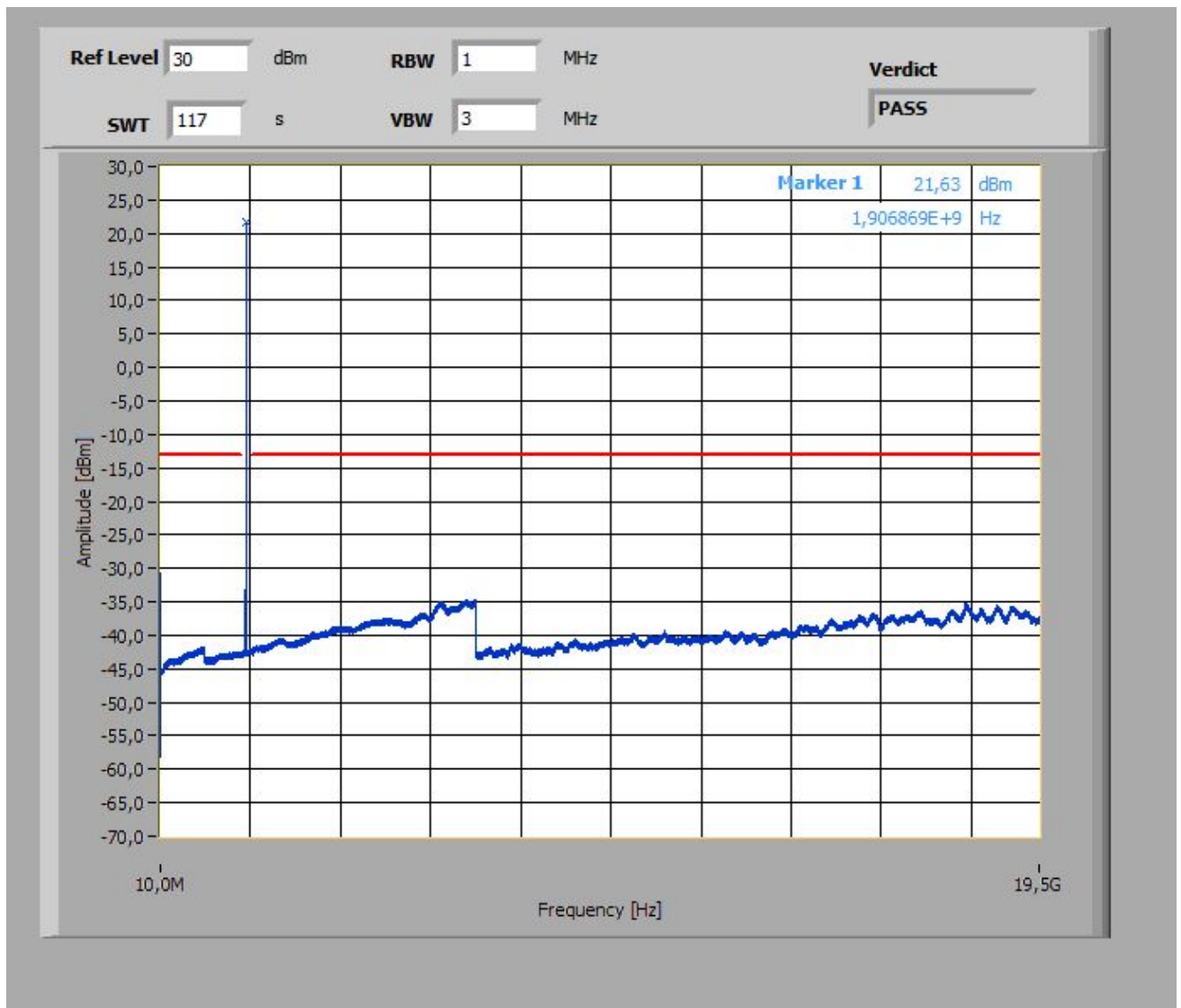
Plot 3: Channel 9538 (10 MHz – 19.5 GHz)
