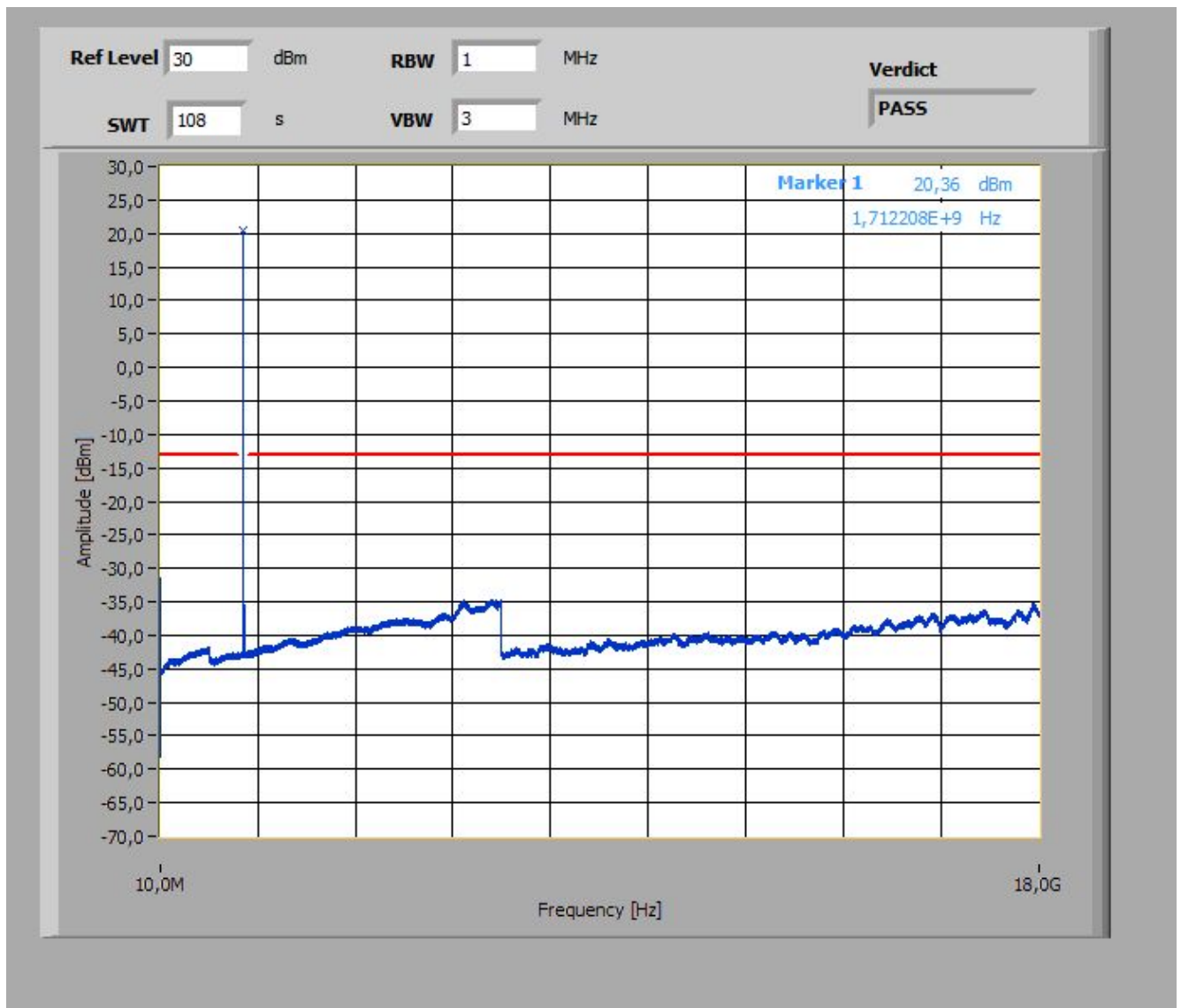
Plot 1: Channel 1312 (10 MHz - 18 GHz)
