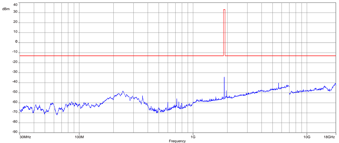
Plot 2: Channel 9400 (30 MHz – 18 GHz)
