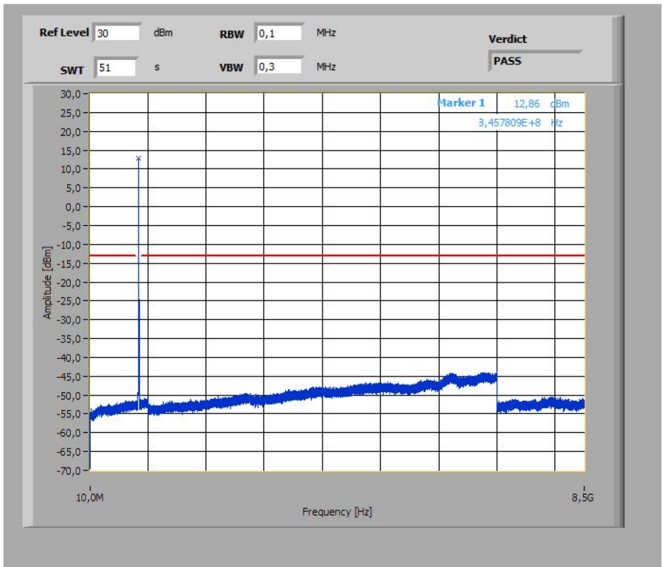
Plot 3: Channel 4233 (10 MHz – 8.5 GHz)
