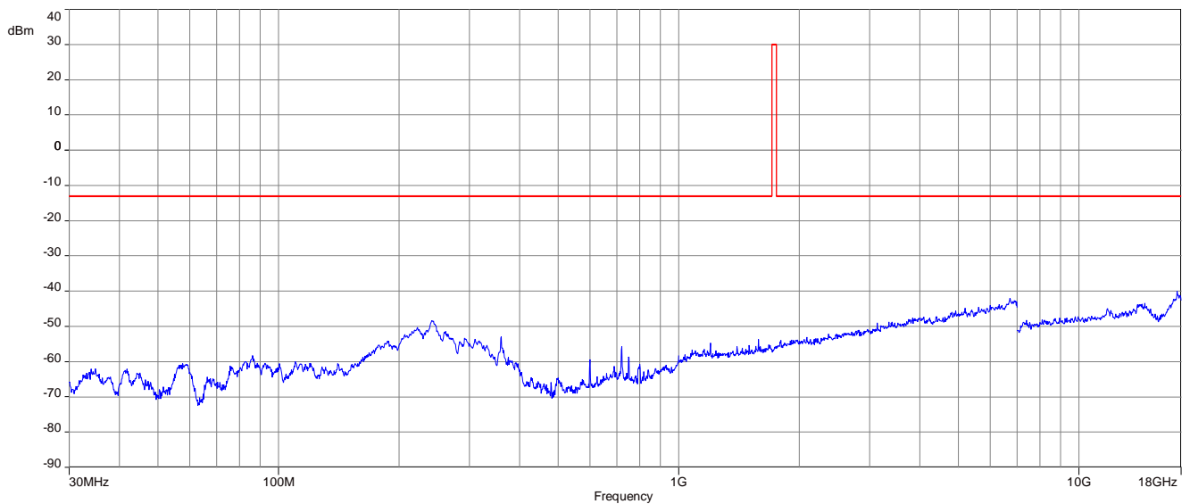
Plot 2: Channel 1412 (30 MHz – 18 GHz)
