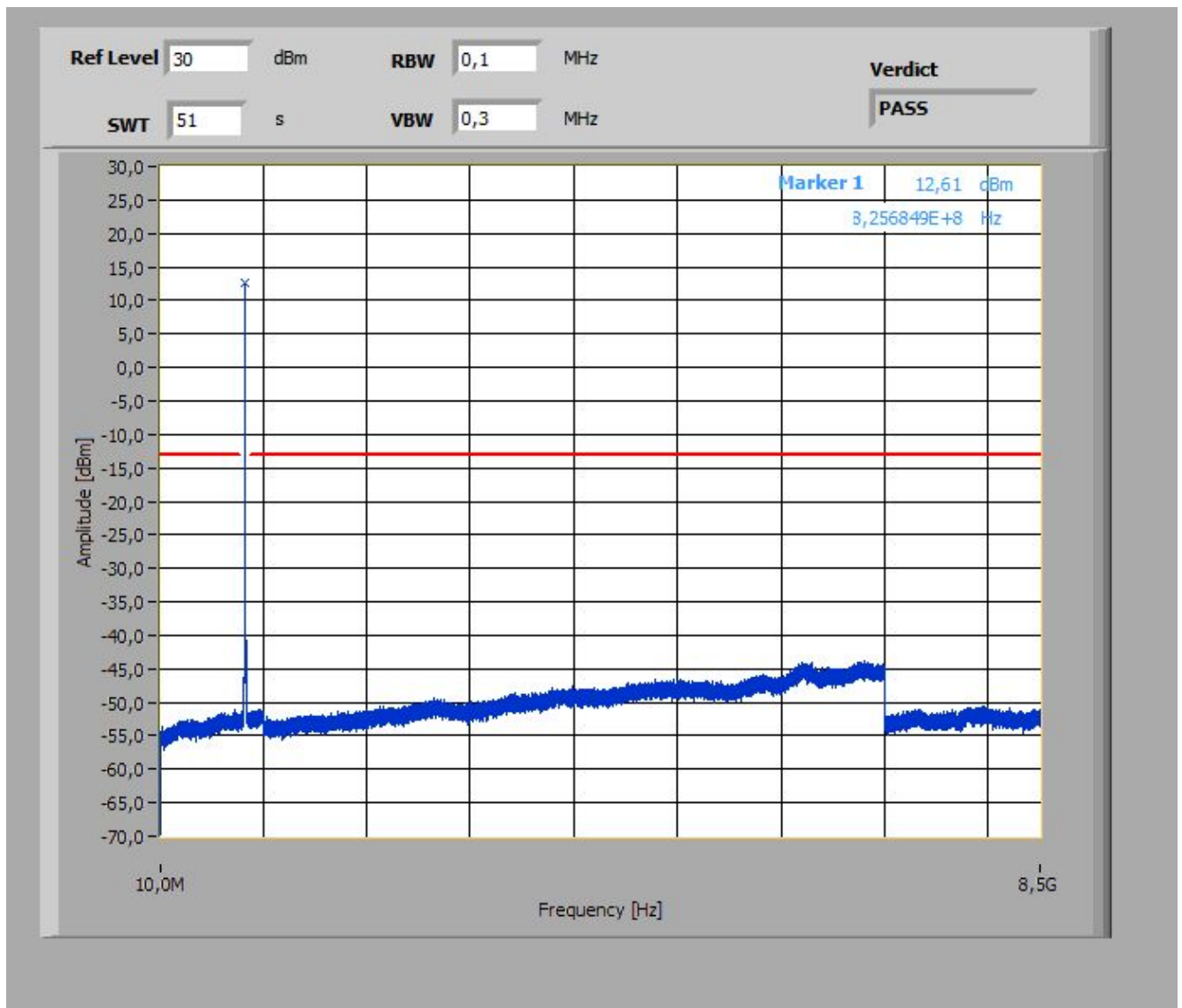
Plot 1: Channel 4132 (10 MHz – 8.5 GHz)
