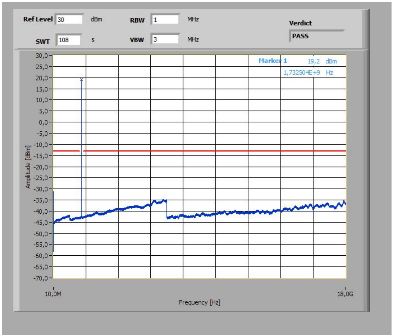
Plot 2: Channel 1412 (10 MHz - 18 GHz)
