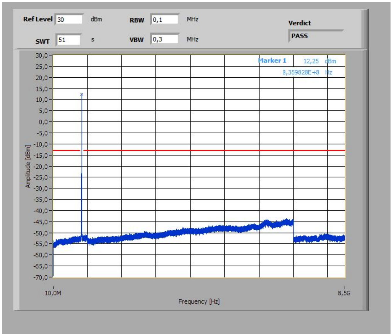
Plot 2: Channel 4180 (10 MHz – 8.5 GHz)
