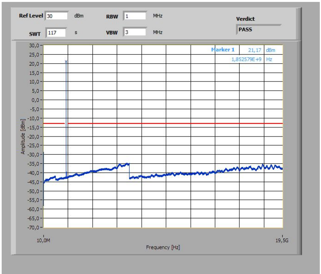
Plot 1: Channel 9262 (10 MHz – 19.5 GHz)
