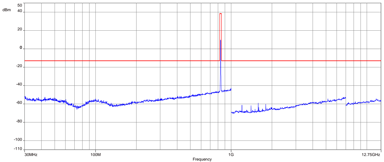
Plot 2: Channel 4180 (30 MHz – 12.75 GHz)
