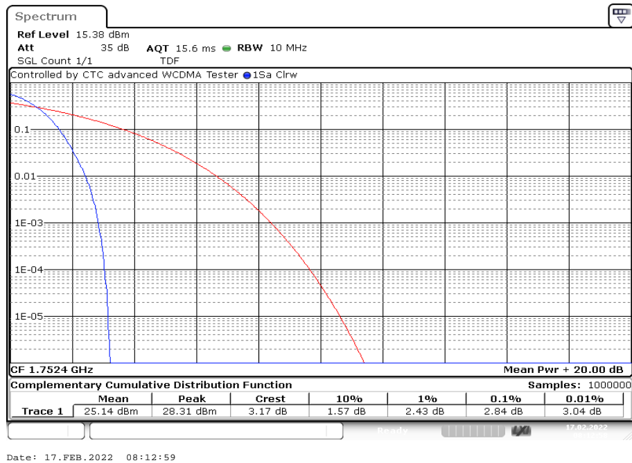
Plot 3: CCDF, channel 1513
