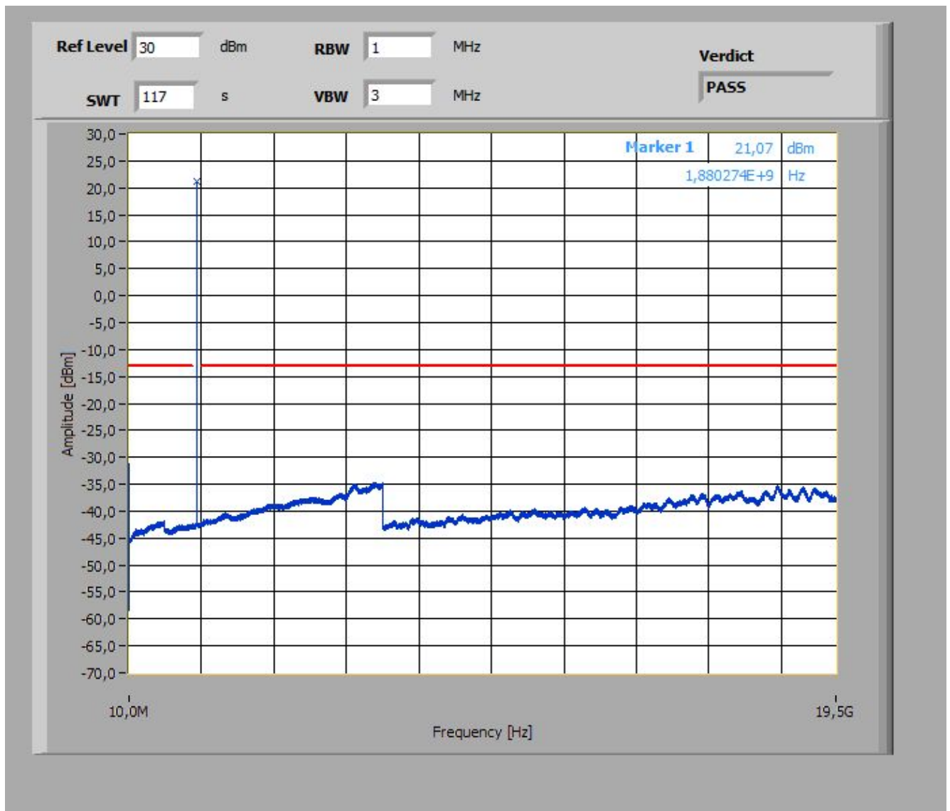
Plot 2: Channel 9400 (10 MHz – 19.5 GHz)
