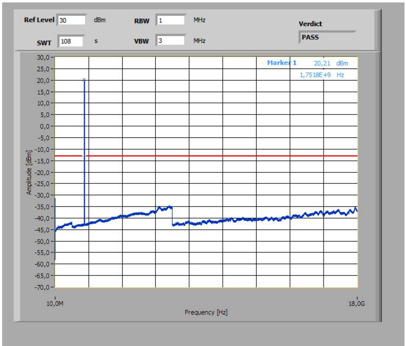
Plot 3: Channel 1513 (10 MHz - 18 GHz)
