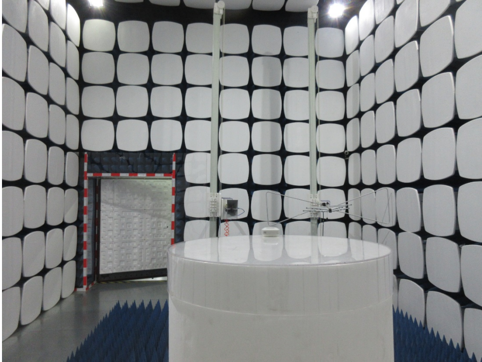
Radiated Emissions which fall in the restricted bands & Radiated Emissions
