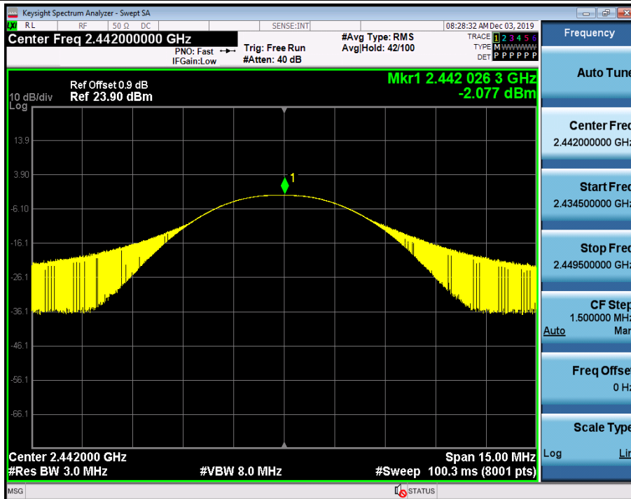
Maximum peak conducted output power_BLE_2442_Ant1
