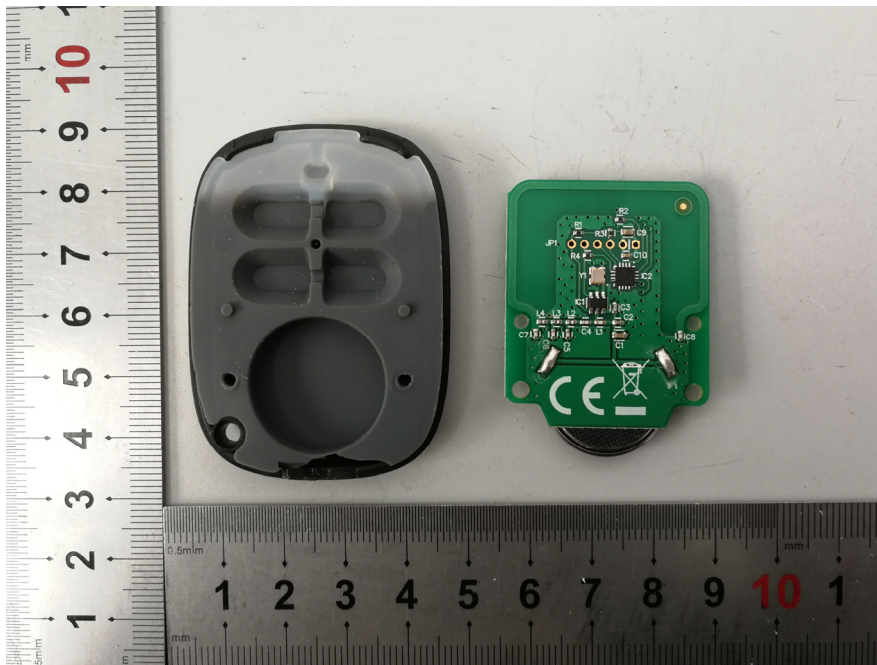
EUT – Cover Removed View-2
