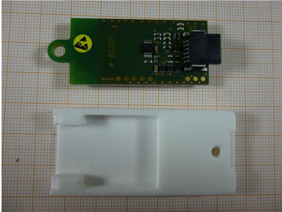
Photo 3 (EUT – internal arrangement):
