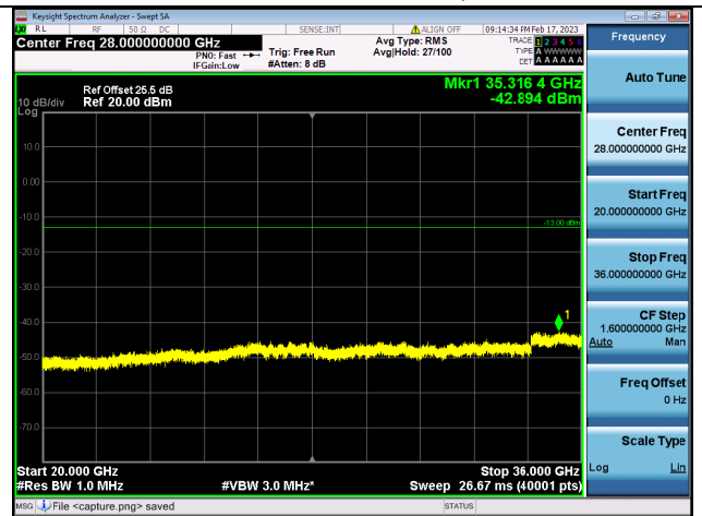
Band42C(3450~3550)-20G-36G / 15MHz+20MHz / 75RB+100RB/ QPSK / Mid CH
