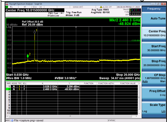
Band42C(3450~3550)-30M-20G / 15MHz+20MHz / 75RB+100RB/ QPSK / High CH
