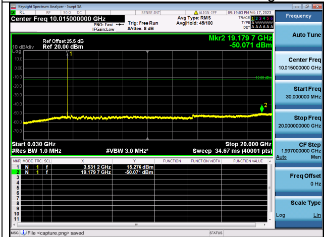
Band42C(3450~3550)-30M-20G / 5MHz+20MHz / 1RB+1RB/ QPSK / High CH
