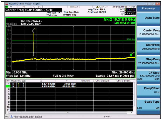
Band42C(3450~3550)-30M-20G / 15MHz+20MHz / 75RB+100RB/ QPSK / Mid CH
