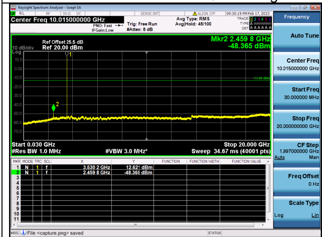
Band42C(3450~3550)-30M-20G / 15MHz+20MHz / 1RB+1RB/ QPSK / High CH
