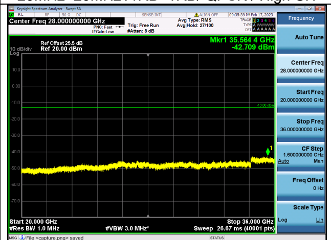
Band42C(3450~3550)-20G-36G / 20MHz+20MHz / 100RB+100RB/ QPSK / High CH
