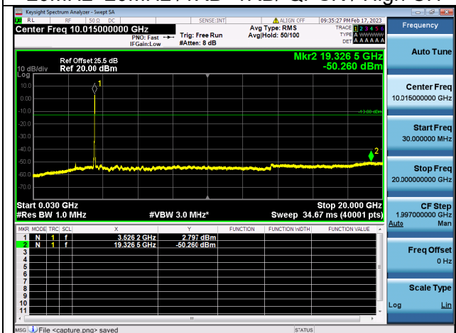
Band42C(3450~3550)-30M-20G / 20MHz+20MHz / 100RB+100RB/ QPSK / High CH
