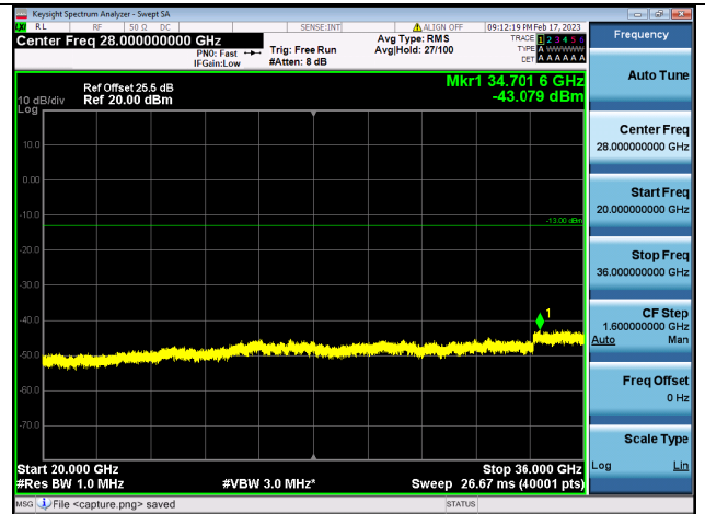
Band42C(3450~3550)-20G-36G / 15MHz+20MHz / 1RB+1RB/ QPSK / Mid CH
