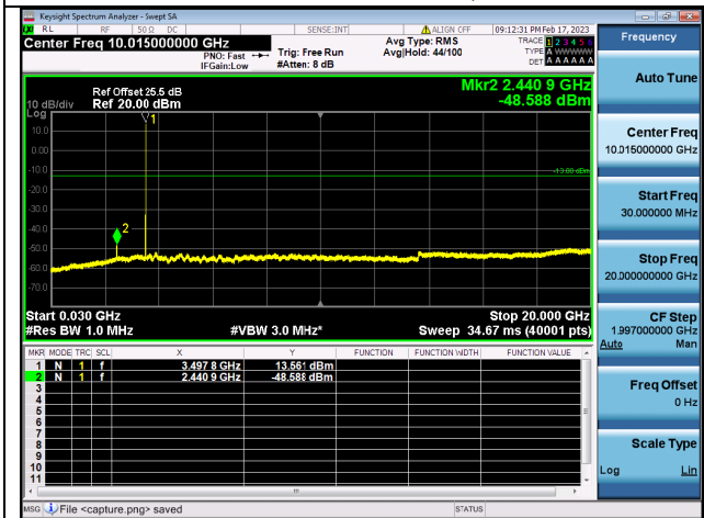
Band42C(3450~3550)-30M-20G / 15MHz+20MHz / 1RB+1RB/ QPSK / Mid CH
