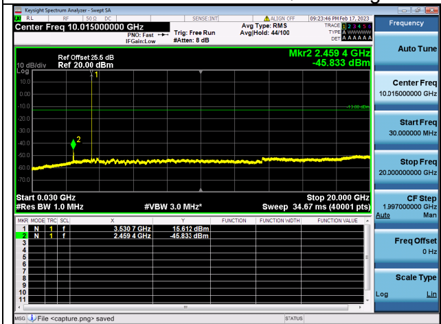
Band42C(3450~3550)-30M-20G / 10MHz+20MHz / 1RB+1RB/ QPSK / High CH
