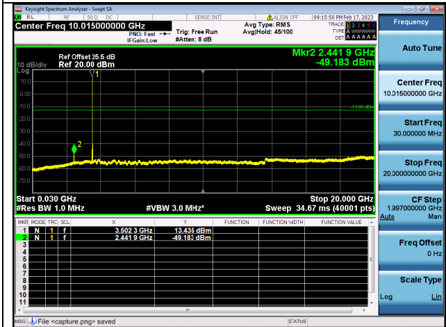
Band42C(3450~3550)-30M-20G / 20MHz+15MHz / 1RB+1RB/ QPSK / Mid CH
