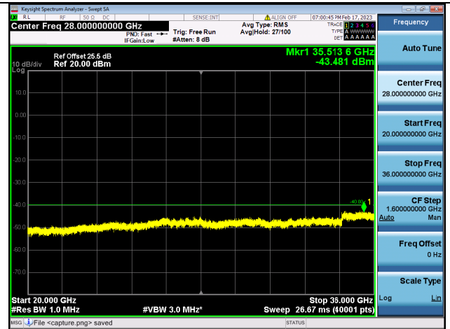
Band42C(3550~3600)-20G-36G / 10MHz+20MHz / 1RB+1RB/ QPSK / Low CH
