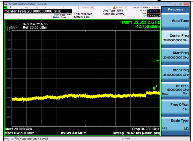
Band42C(3450~3550)-20G-36G / 5MHz+20MHz / 1RB+1RB/ QPSK / High CH
