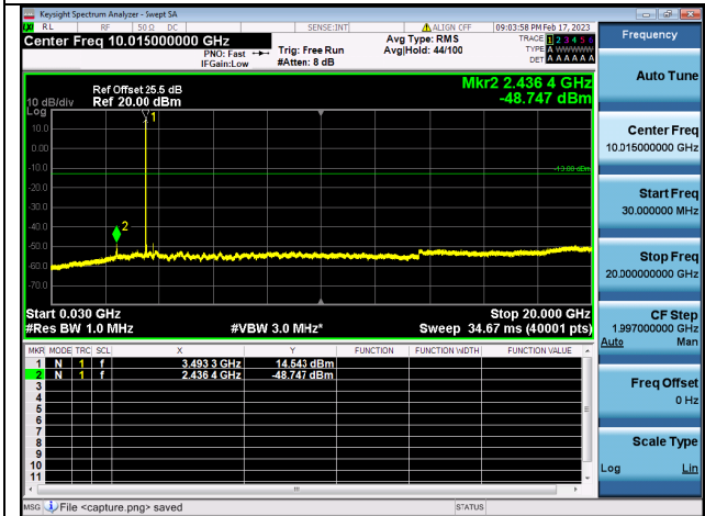
Band42C(3450~3550)-30M-20G / 5MHz+20MHz / 1RB+1RB/ QPSK / Mid CH
