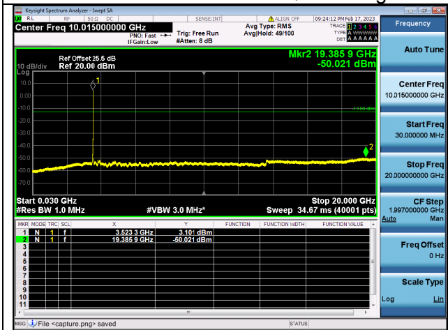
Band42C(3450~3550)-30M-20G / 10MHz+20MHz / 50RB+100RB/ QPSK / High CH
