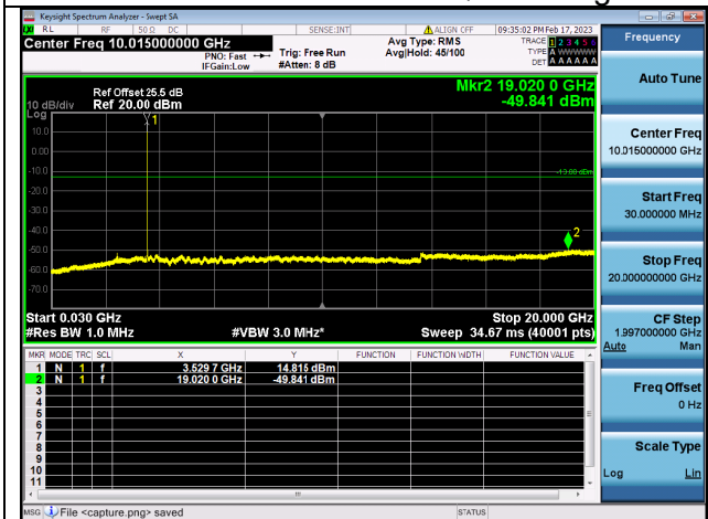
Band42C(3450~3550)-30M-20G / 20MHz+20MHz / 1RB+1RB/ QPSK / High CH
