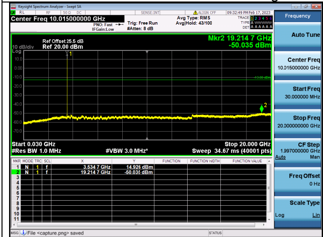
Band42C(3450~3550)-30M-20G / 20MHz+15MHz / 1RB+1RB/ QPSK / High CH
