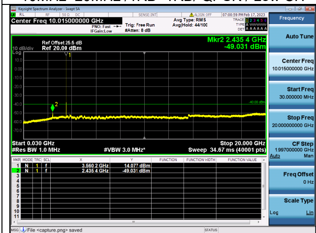
Band42C(3550~3600)-30M-20G / 10MHz+20MHz / 1RB+1RB/ QPSK / Low CH
