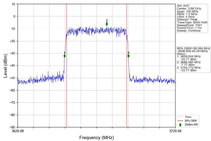
n48_30kHz_SISO_NTNV_40MHz_CP-OFDM 256 QAM_3679.98MHz_Outer_Full
