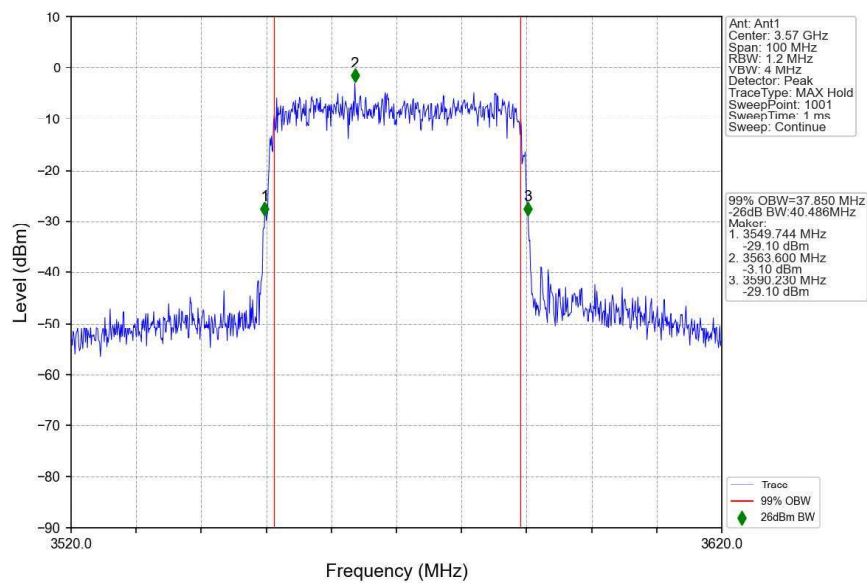
n48_30kHz_SISO_NTNV_40MHz_CP-OFDM 16 QAM_3570MHz_Outer_Full
