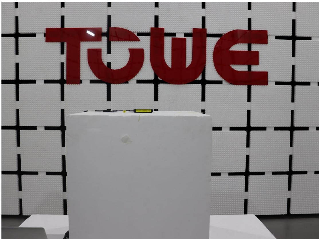
Radiated Spurious Emissions (Above 18000MHz)
