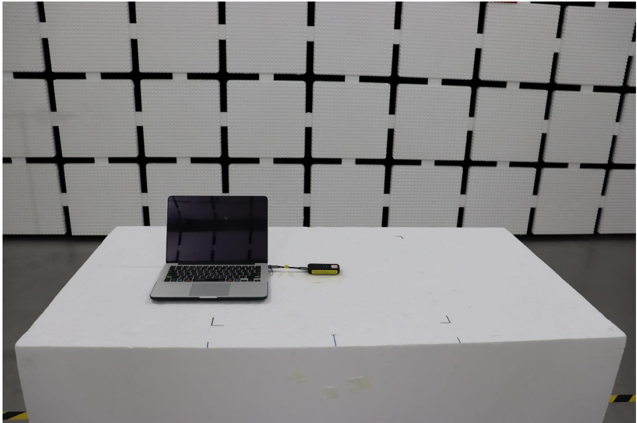
Radiated Spurious Emissions (9kHz to 30MHz)
