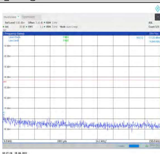
1-N77-3700-3980--30-100-H-1-DFT-QPSK-Edge_1R B_Left-1@0-0.009-0.15-Ant2--77.35--43-PASS
