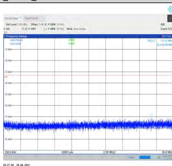
1-N77-3700-3980--30-100-H-1-DFT-QPSK-Edge_1R B_Left-1@0-0.15-30-Ant2--71.15--33-PASS
