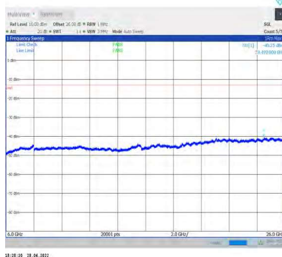
1-N77-3700-3980--30-100-H-1-DFT-QPSK-Edge_1R B_Left-1@0-6000-26000-Ant2--40.25--13-PASS
