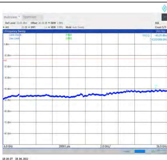
1-N77-3700-3980--30-100-M-1-DFT-QPSK-Edge_1R B_Left-1@0-6000-26000-Ant2--40.28--13-PASS
